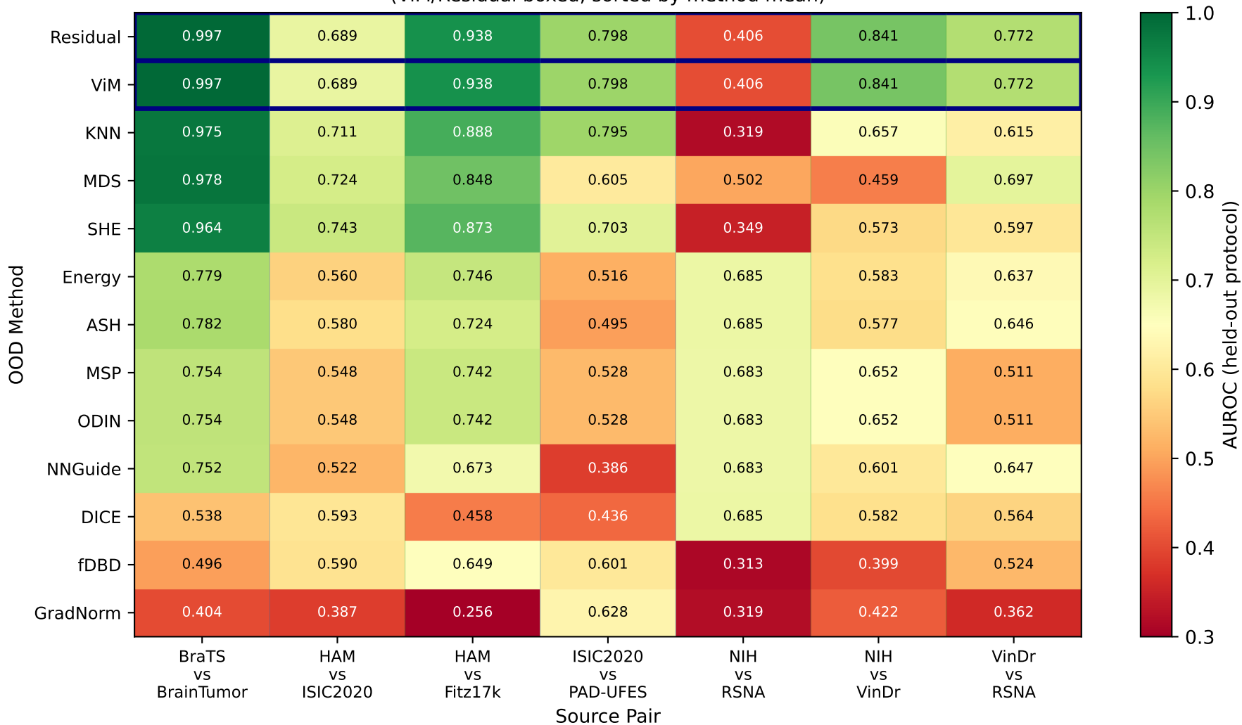
13-Method \times 7-Pair Held-out AUROC Heatmap (ViM/Residual boxed; sorted by method mean)
