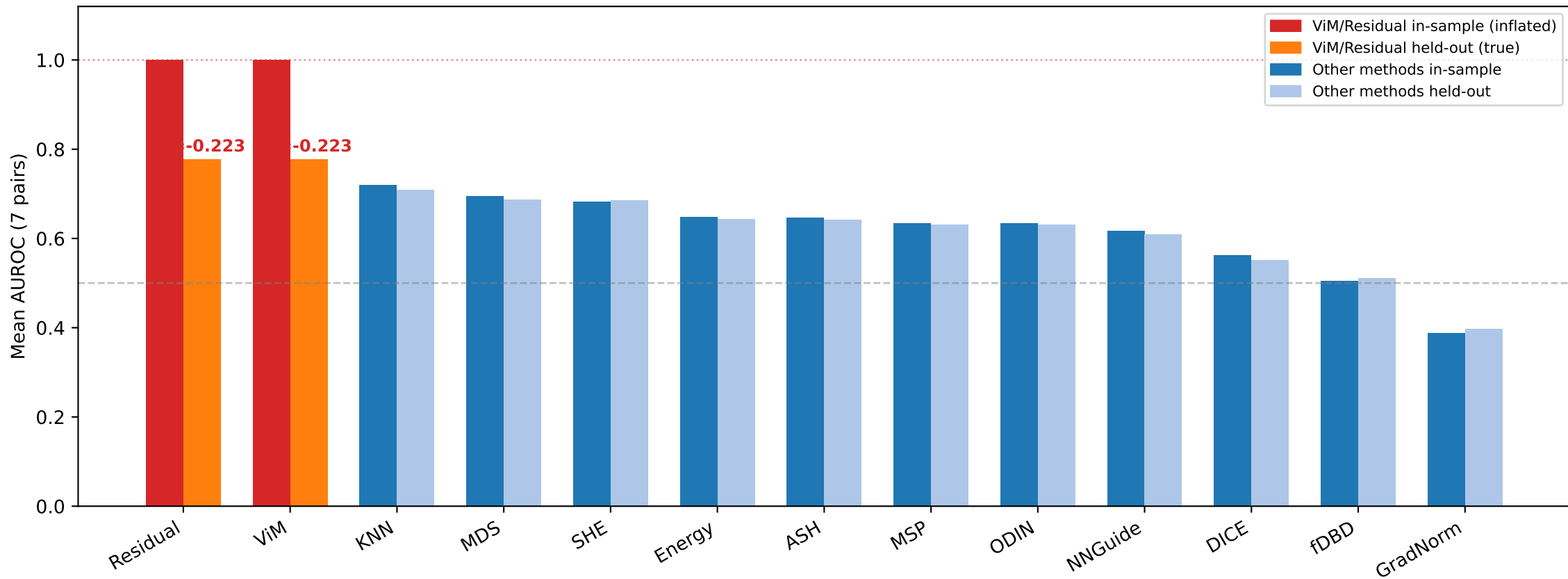
In-sample vs Held-out: 13-method \times 7-pair Mean AUROC (ViM/Residual inflate 1.0 \rightarrow 0.777, others stable)
