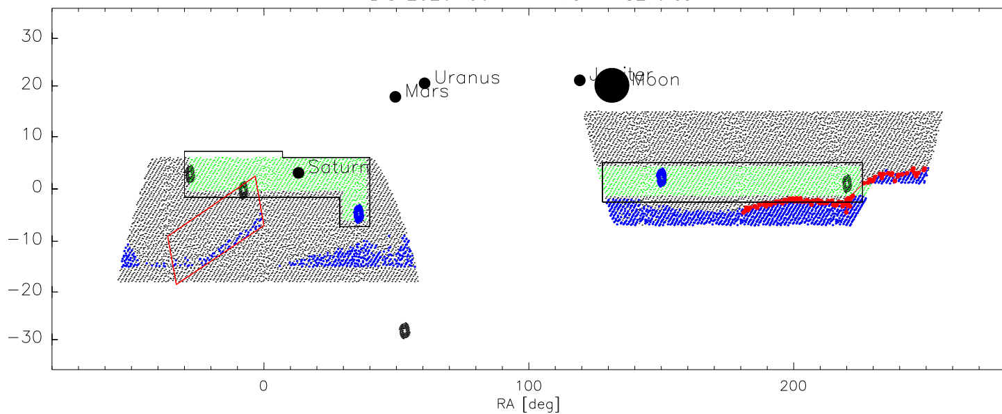
IBIS 2026-06-17A M517 82 tiles
