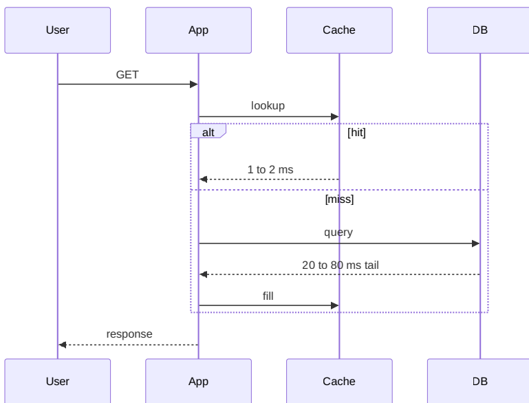
Figure 7.1 — Budget the path. Cache exists to cut database time on hits; it can hurt p99 on stampedes (Chapter 11).
