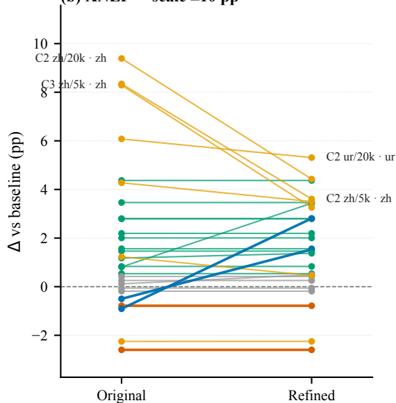
(b) XNLI — scale \pm 10 pp
