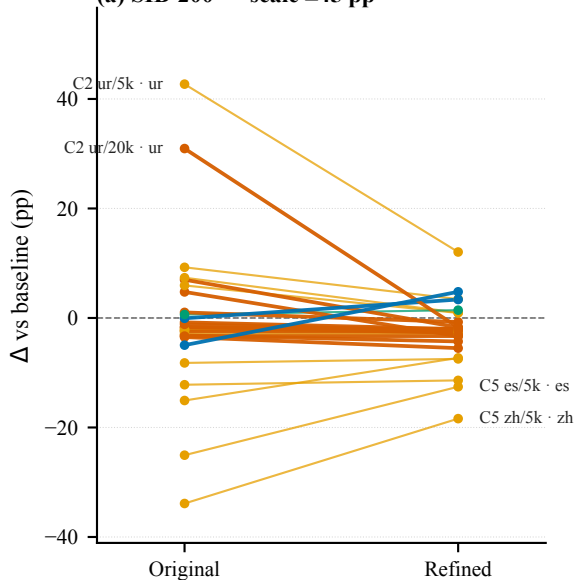
(a) SIB-200 — scale \pm 45 pp
