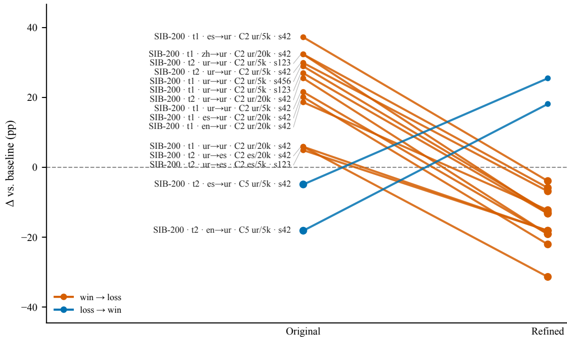
Top 15 of 43 SIB-200 sign-flips by |shift|; rows: benchmark · template · data→instr · condition · seed
