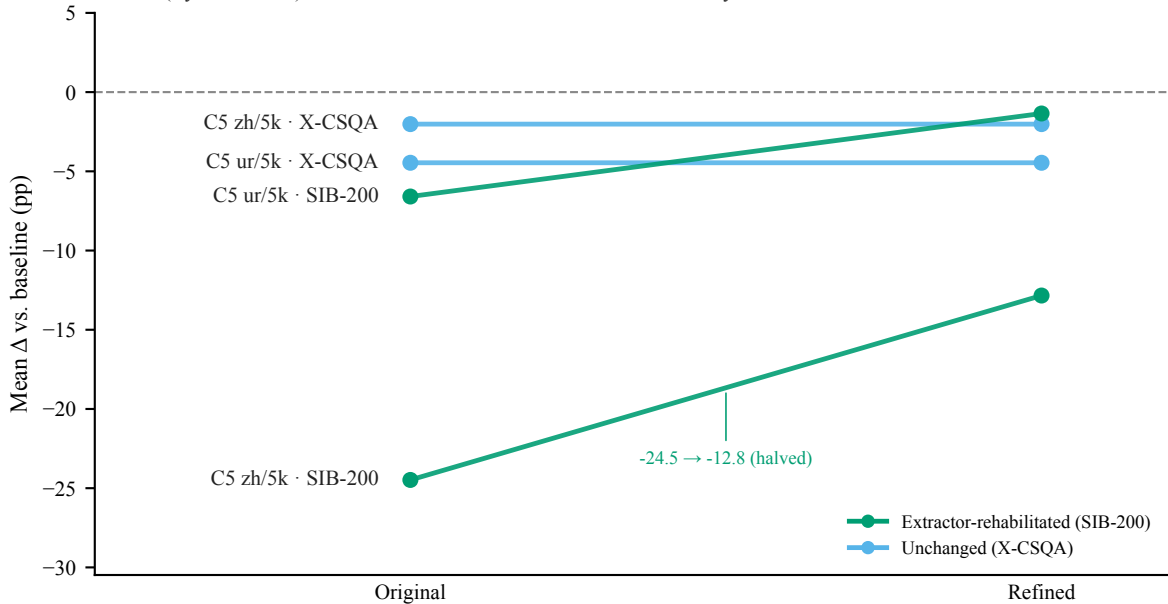
Cond-5 (Aya-translated) vs baseline — extractor effect on the cond-5 story
