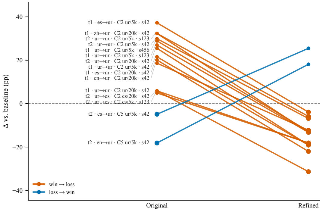
Top 15 sign-flips by magnitude (full 48 in appendix). All flips on SIB-200; rows: template · data→instr · condition · seed
