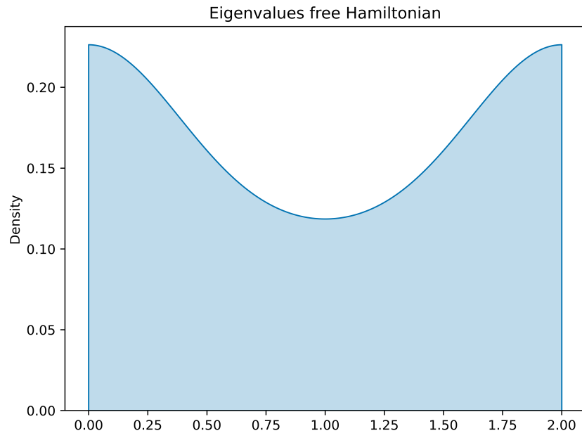
Figure 1: KDE plot of the spectrum of the free Hamiltonian, with L = 1000 and \Delta x = 1 .
