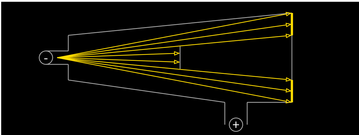
Figure 8: when a cathode-ray collides fluorescent material, it emit light.
