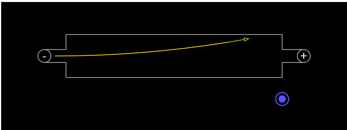
Figure 9: Cathode-rays receive the same force as lorentz force of negative-charge.
