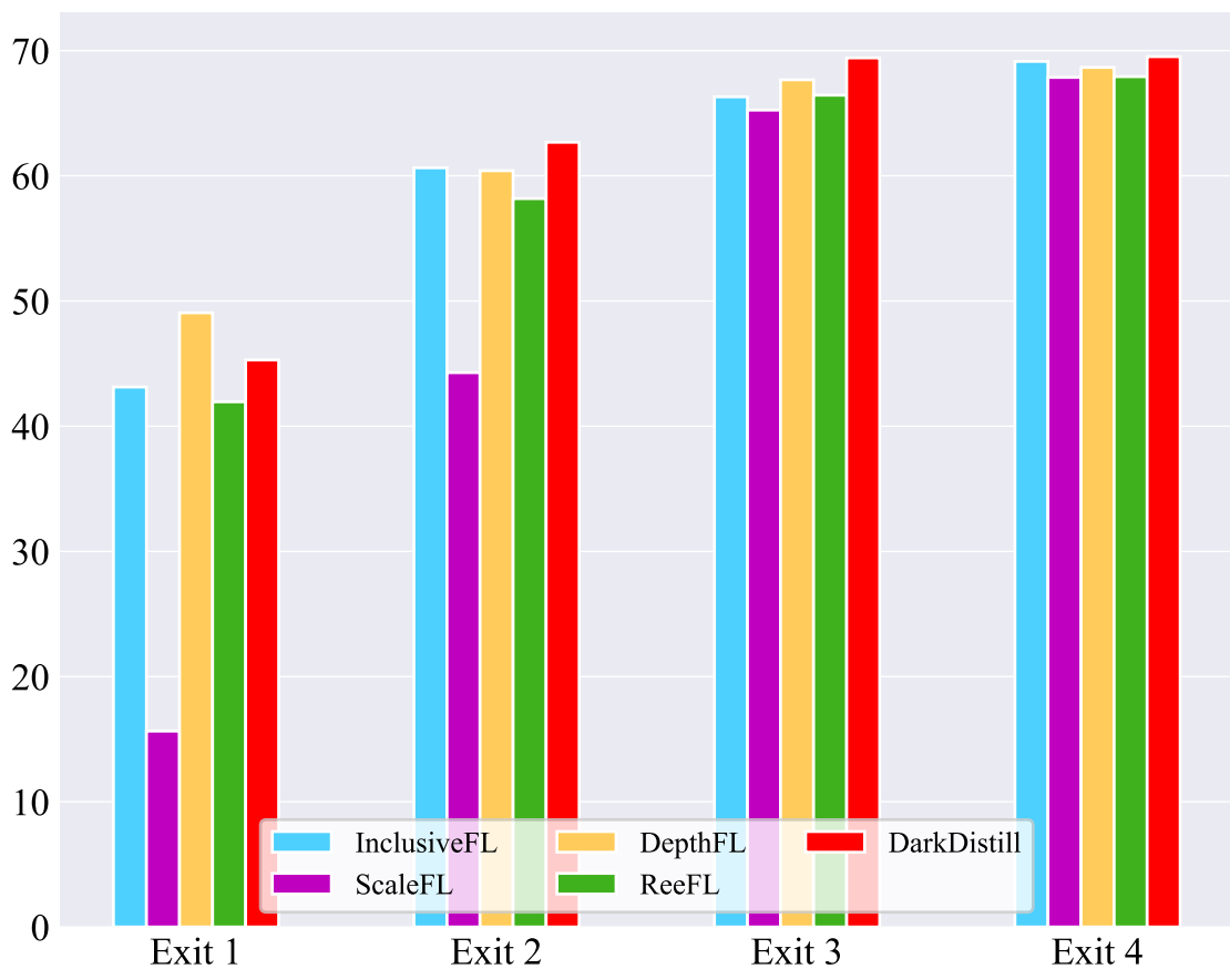
Accuracy (%)
