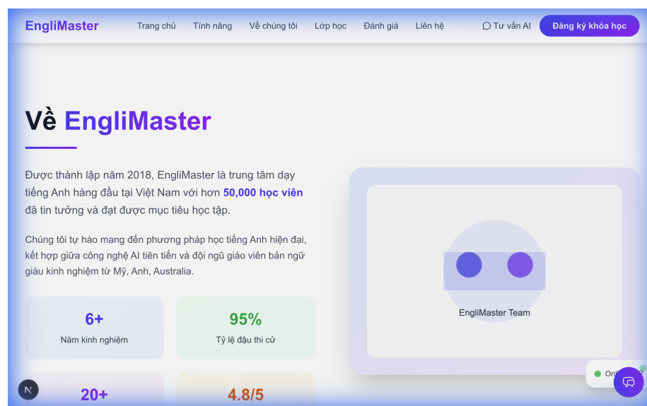
Figure 6: About Section
