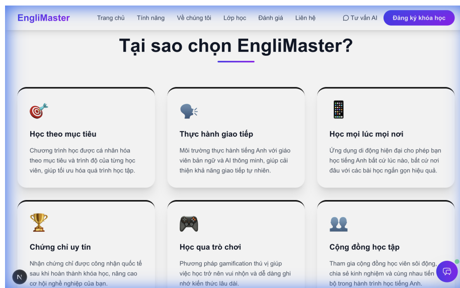
Figure 5: Features Section
