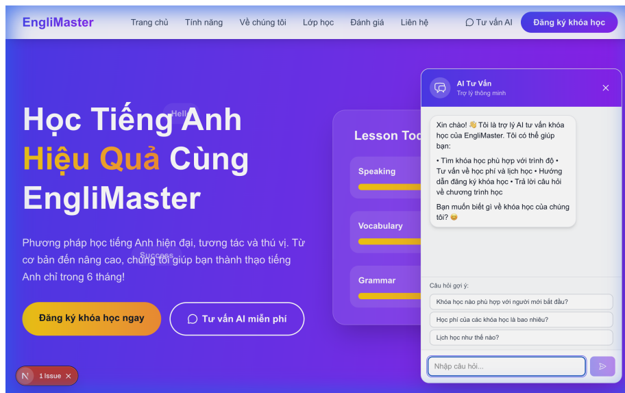
Figure 13: AI Widget
