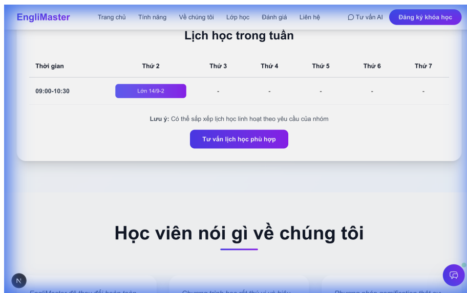
Figure 11: CTA Section
