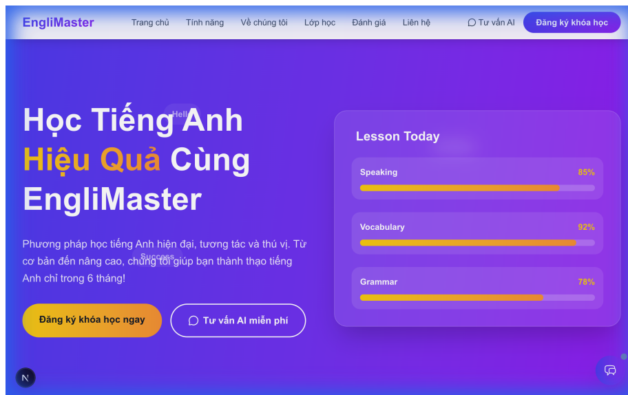
Figure 4: Hero Section
