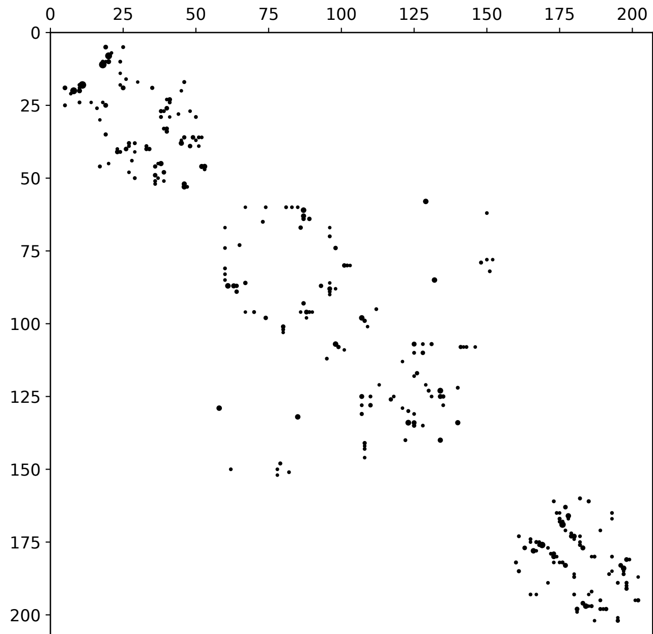
140 evolutionary couplings
