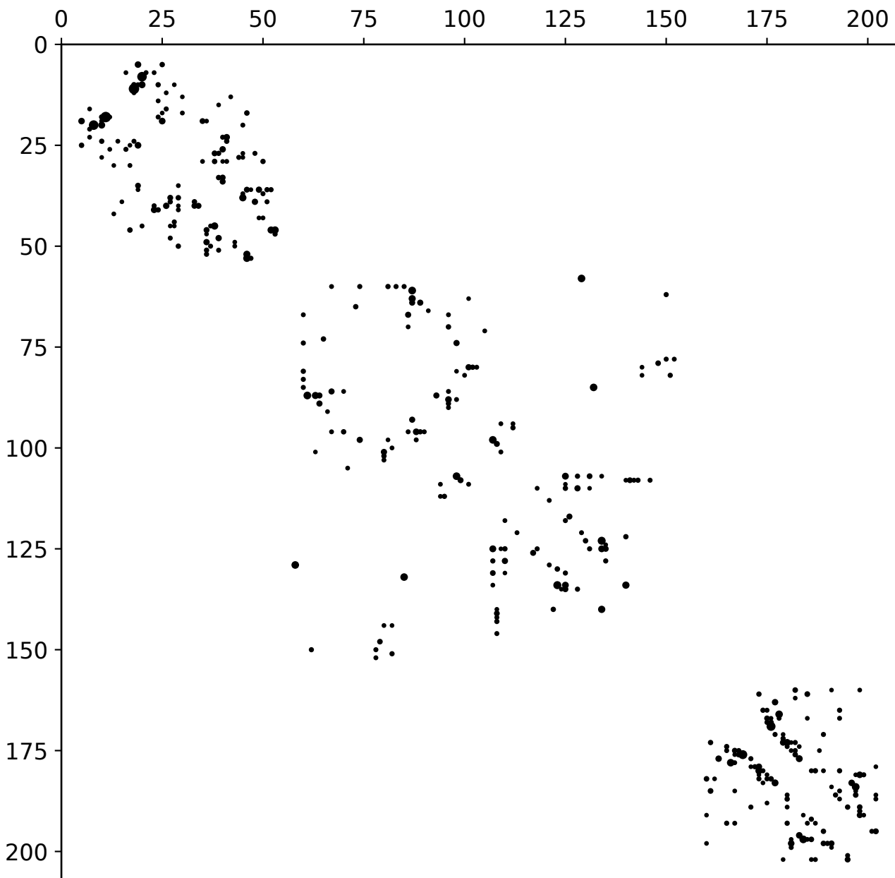
190 evolutionary couplings
