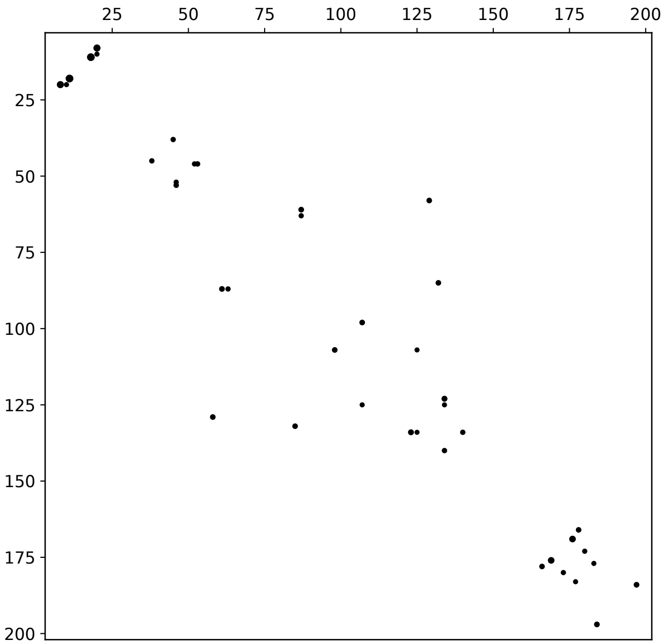
20 evolutionary couplings
