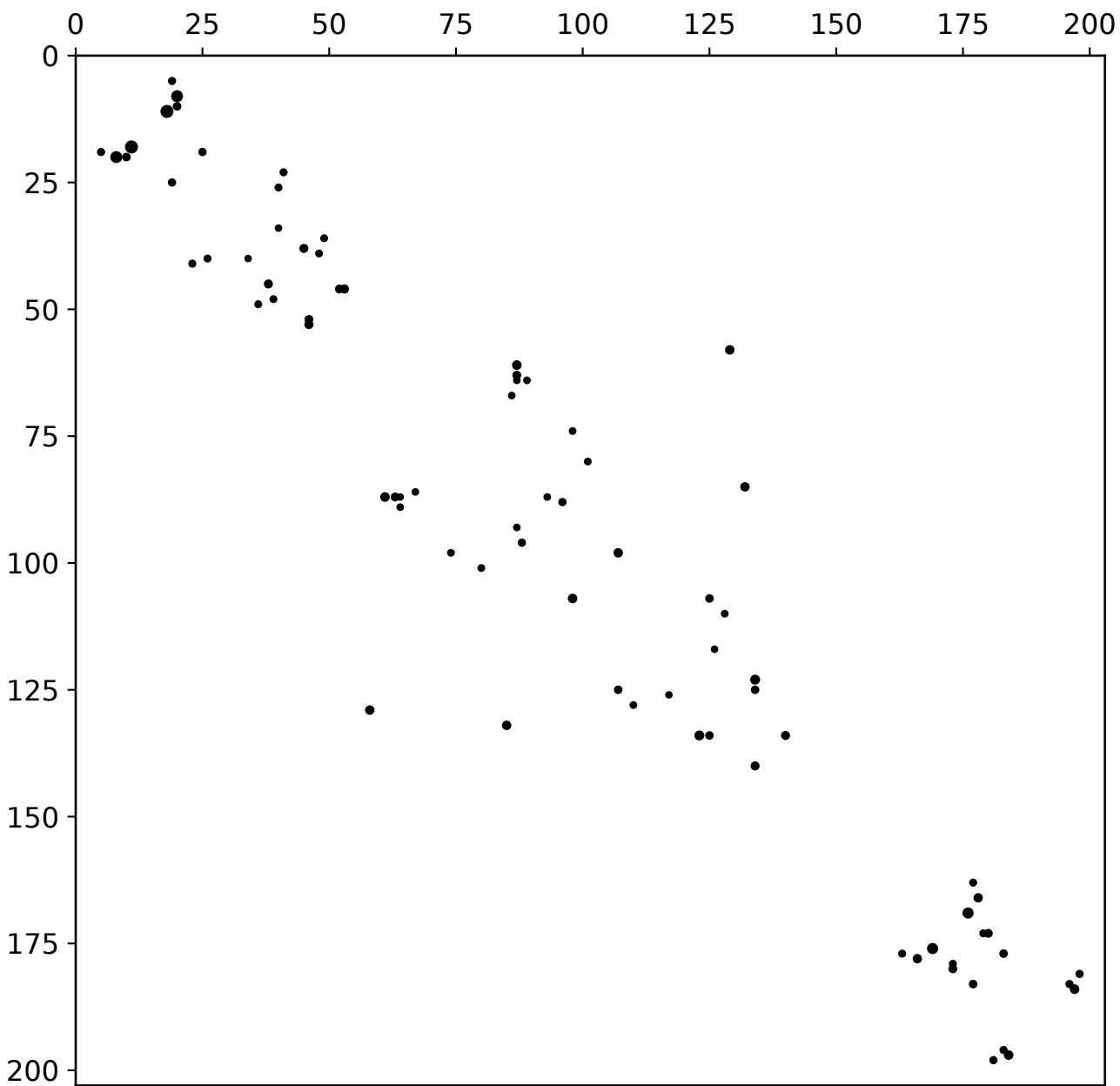
40 evolutionary couplings
