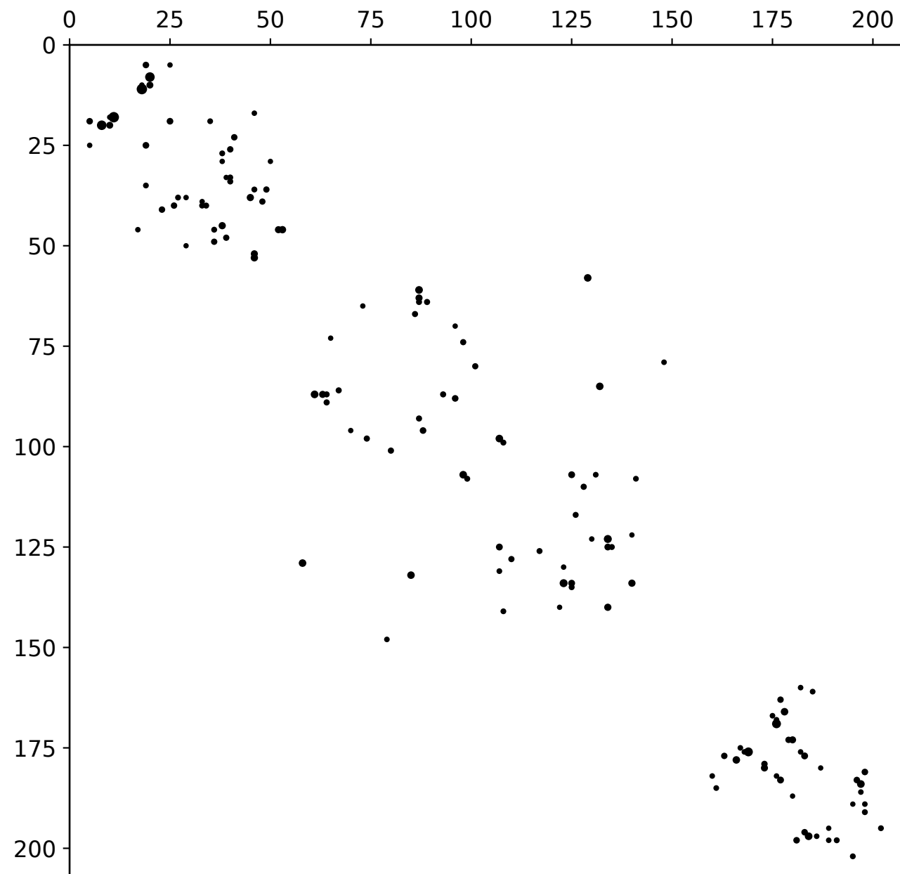
70 evolutionary couplings
