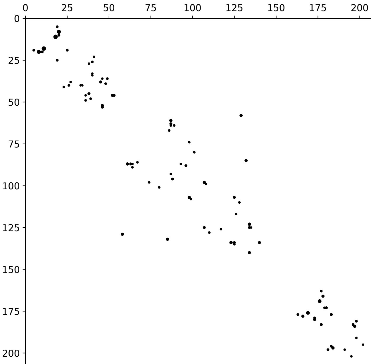
47 evolutionary couplings
