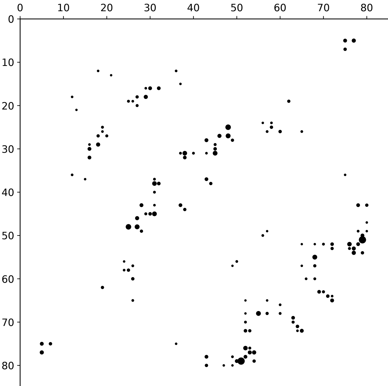
68 evolutionary couplings
