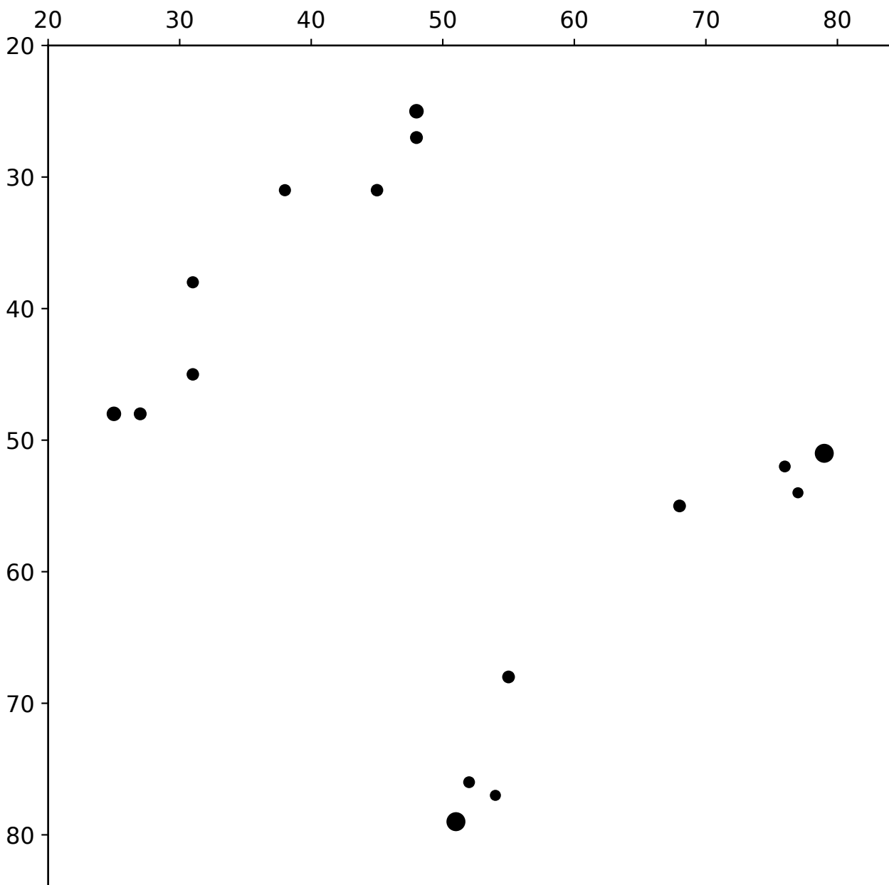
8 evolutionary couplings
