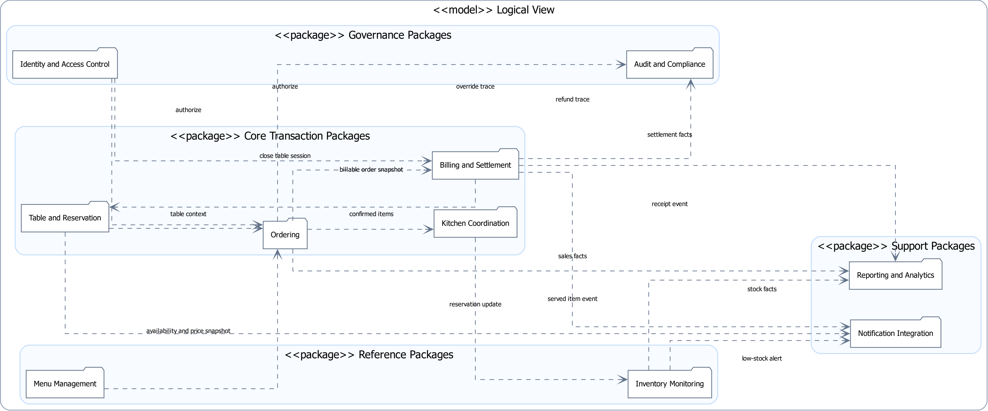
UML Package Diagram - Refined Logical Capability Model of IRMS
