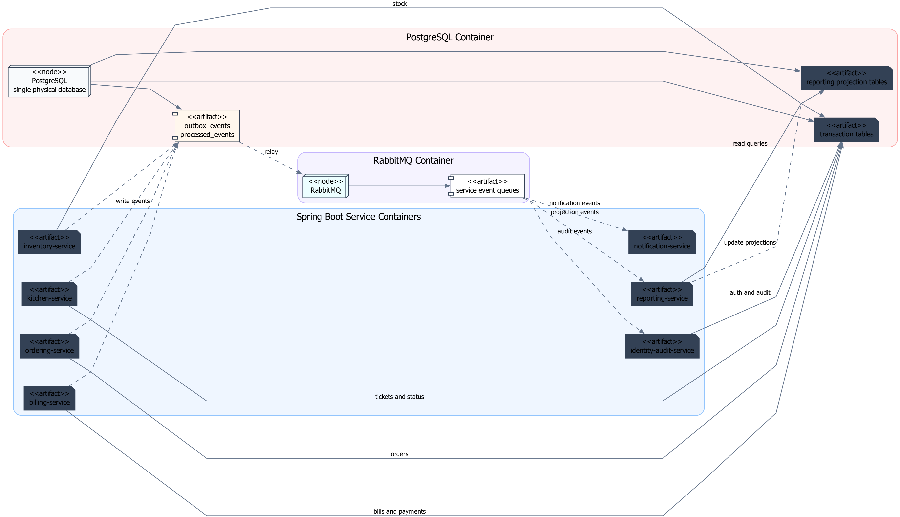
Deployment Diagram - Data and Execution Mapping
