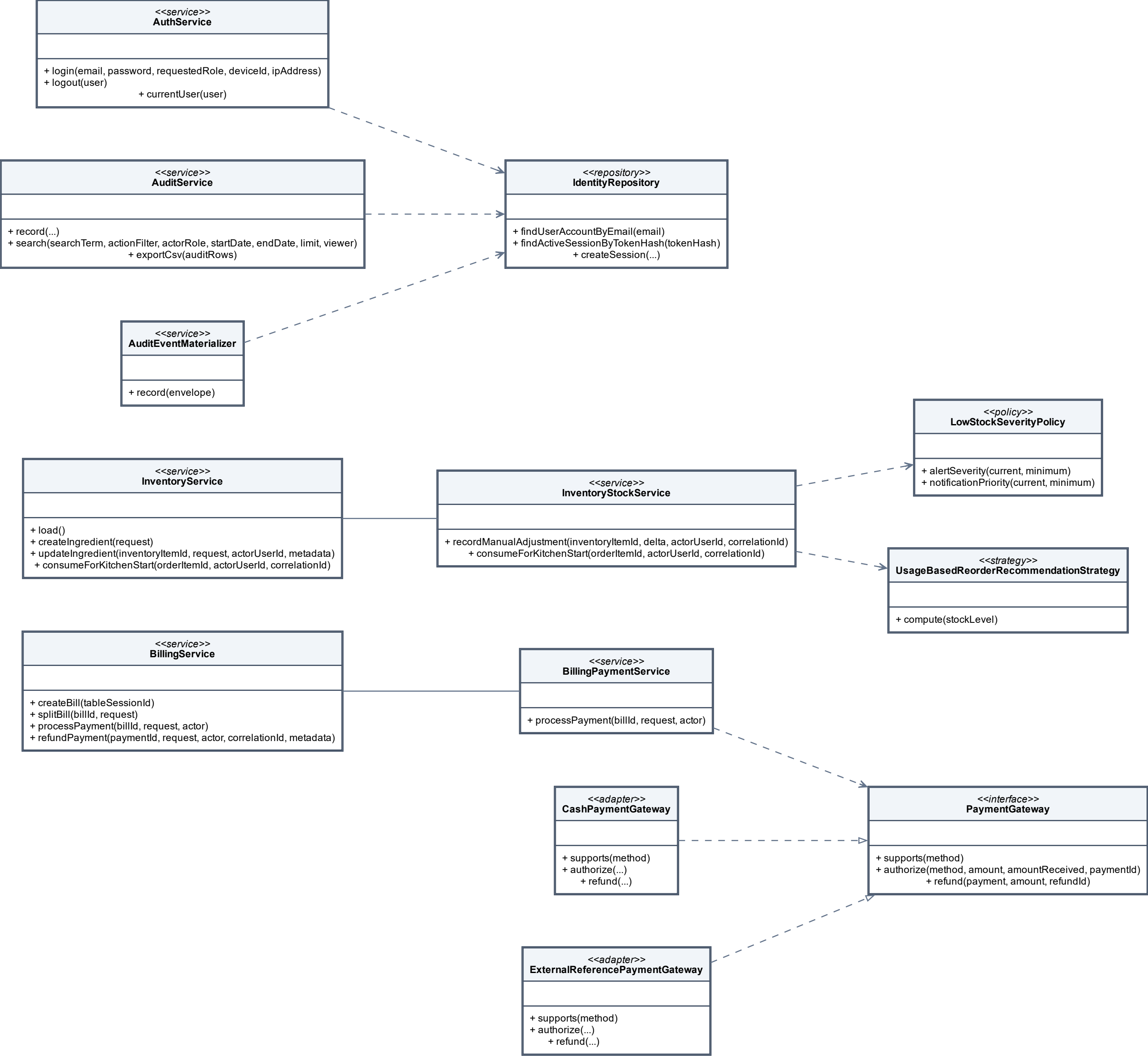
UML Class Diagram - Billing, Inventory and Governance Extension Points
