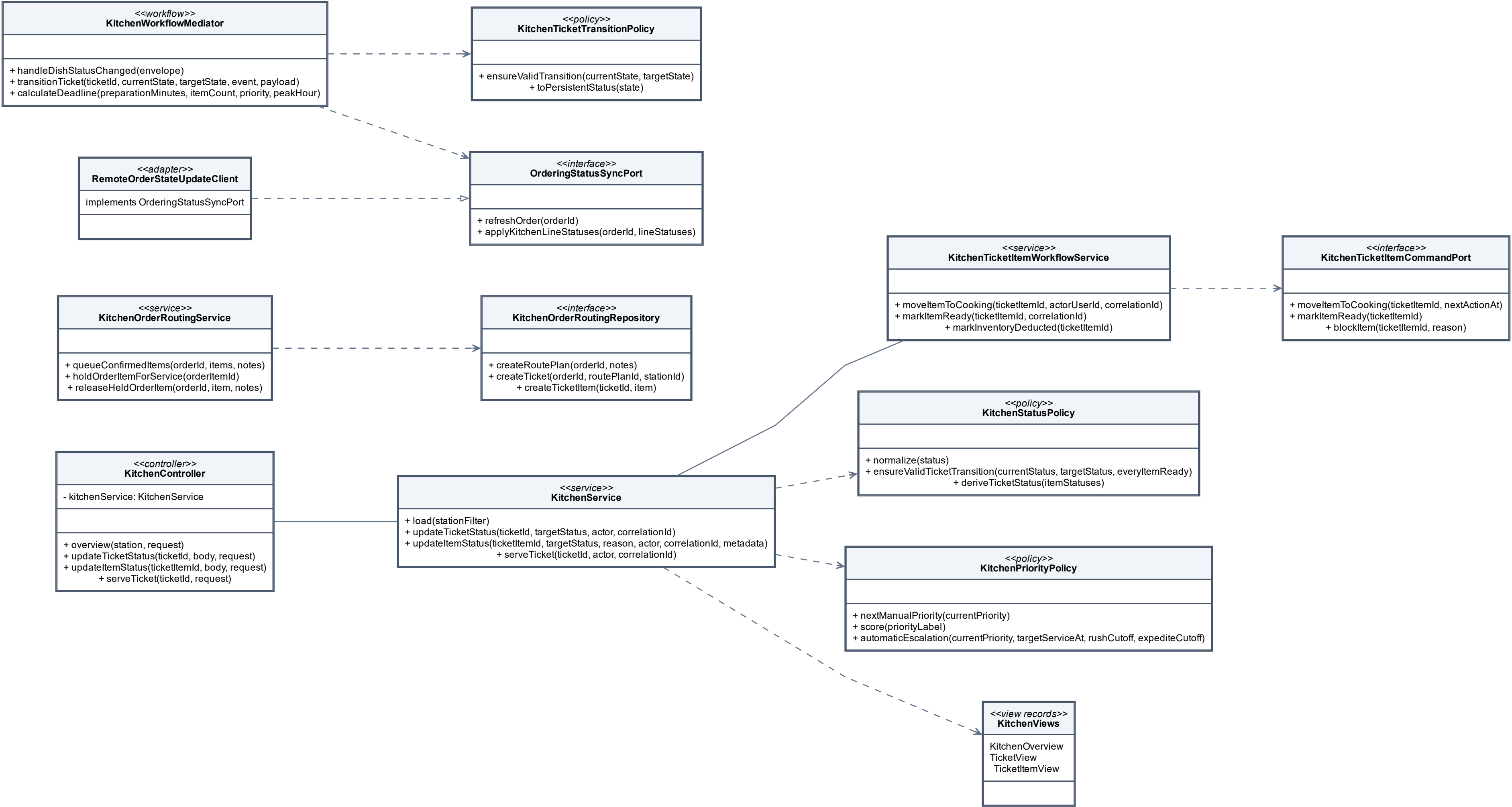
UML Class Diagram - Kitchen Coordination Module Structure
