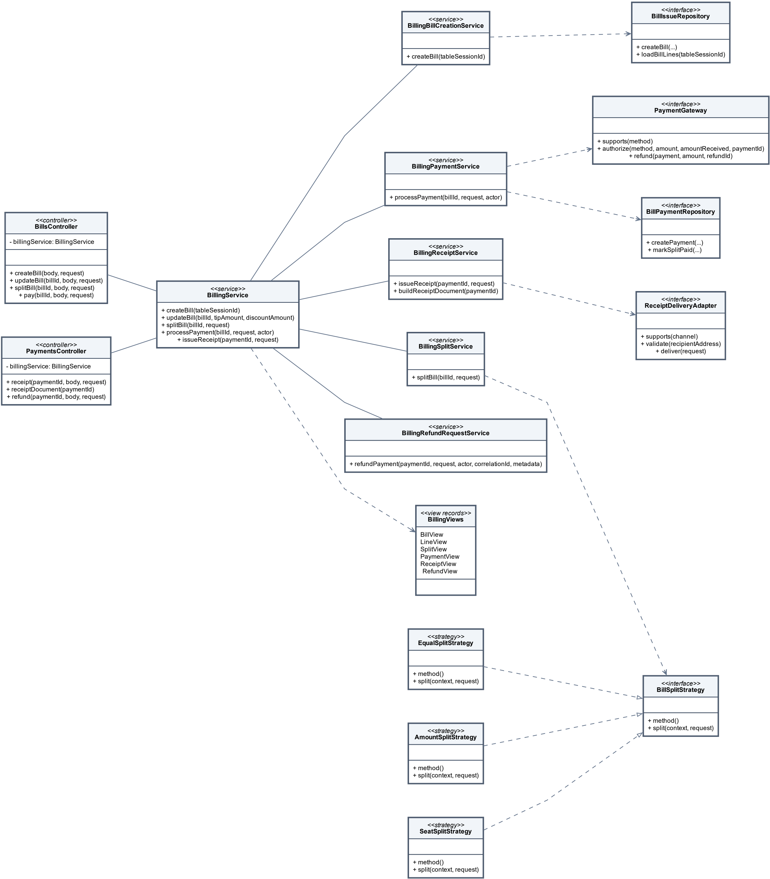
UML Class Diagram - Billing and Settlement Module Structure
