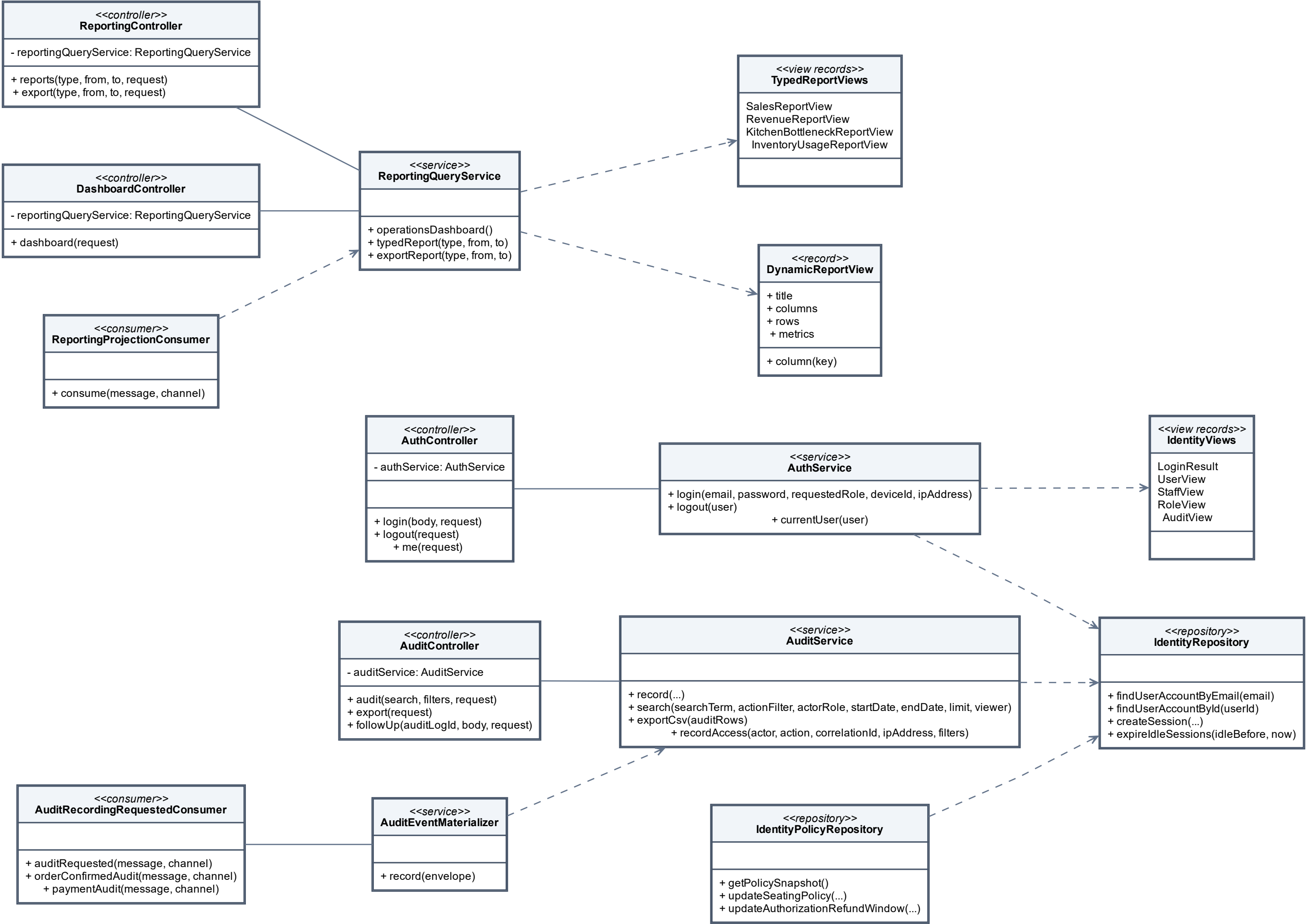
UML Class Diagram - Identity, Audit and Reporting Support
