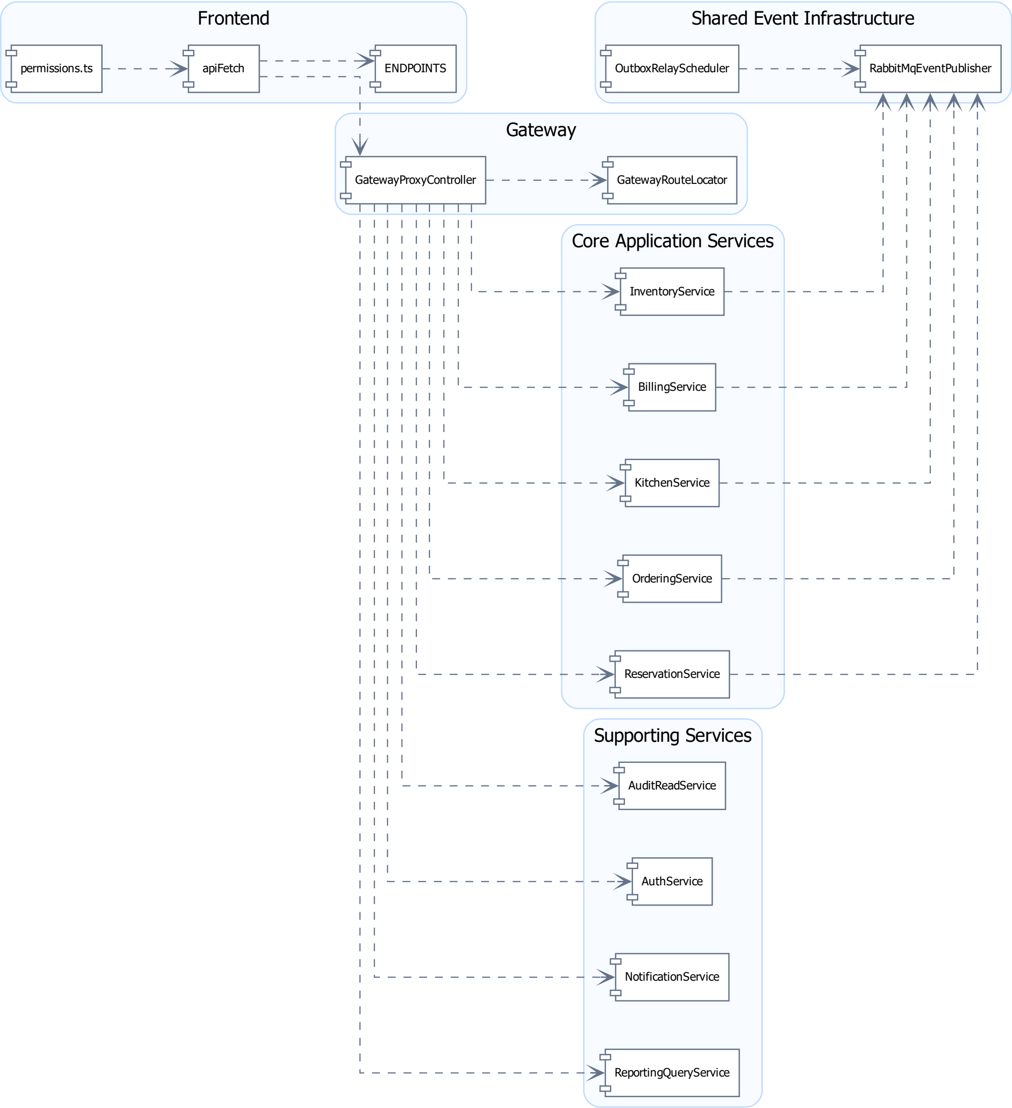
Component Diagram - IRMS Runtime Dependency Overview
