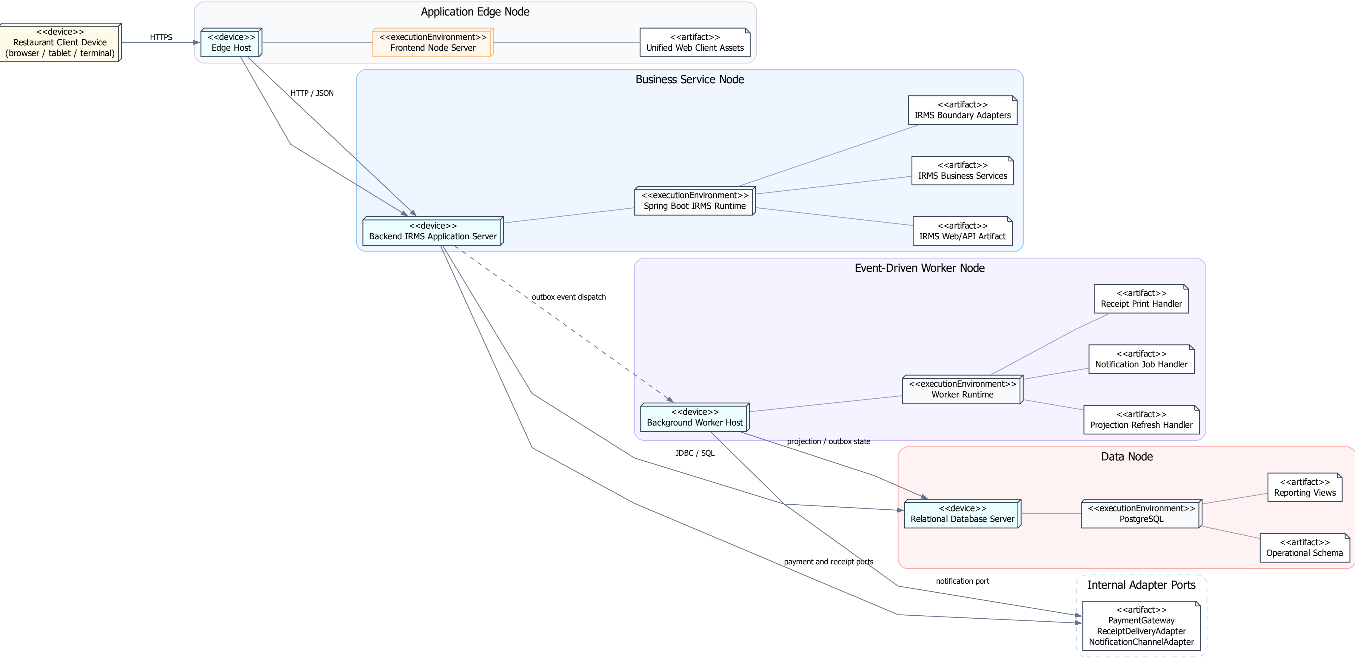
Deployment Diagram - Physical Deployment
