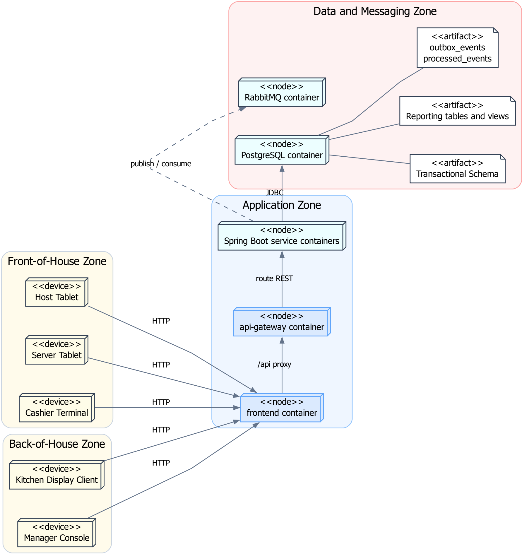
Deployment Diagram - Network Zones and Trust Boundaries
