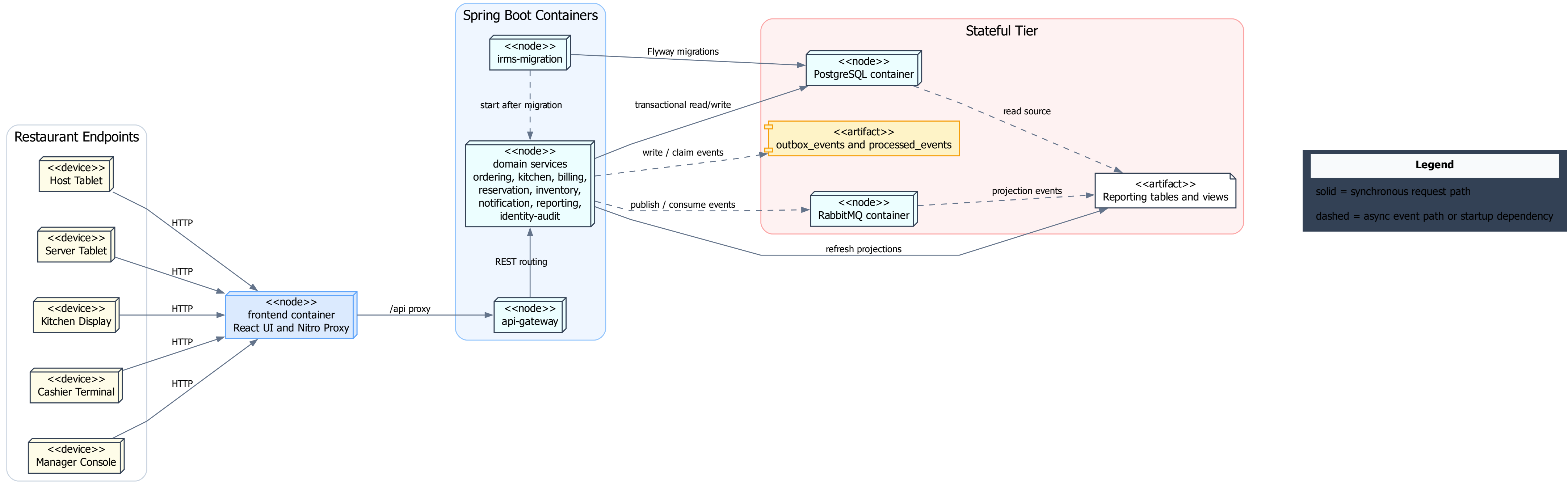
Deployment Diagram - Local Docker Runtime and Failure Isolation
