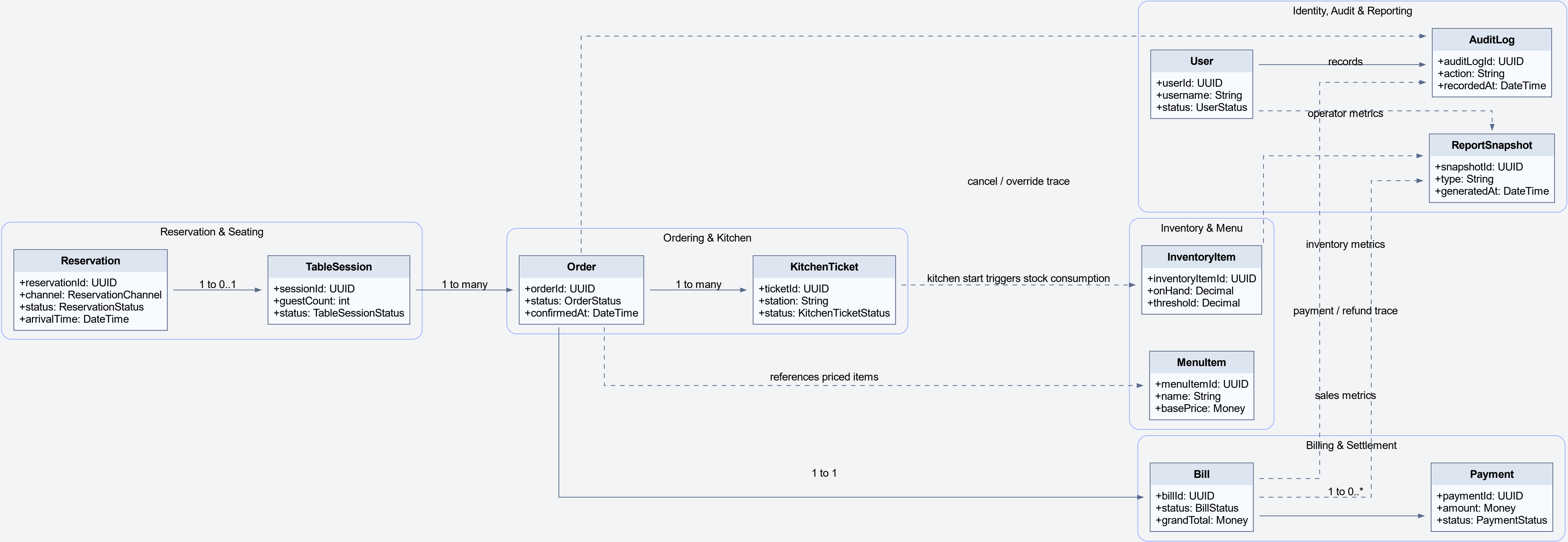
UML Class Diagram - Core Domain Overview
