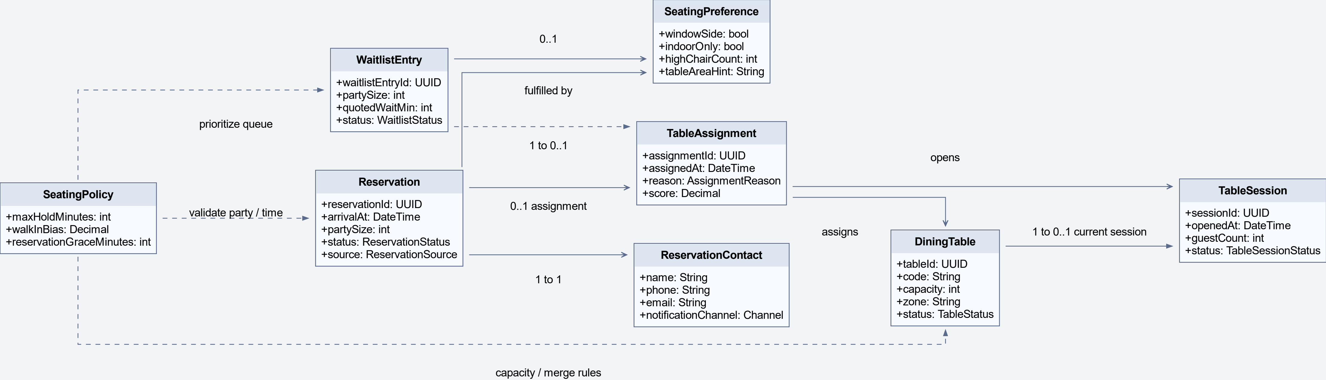
UML Class Diagram - Reservation & Seating Service
