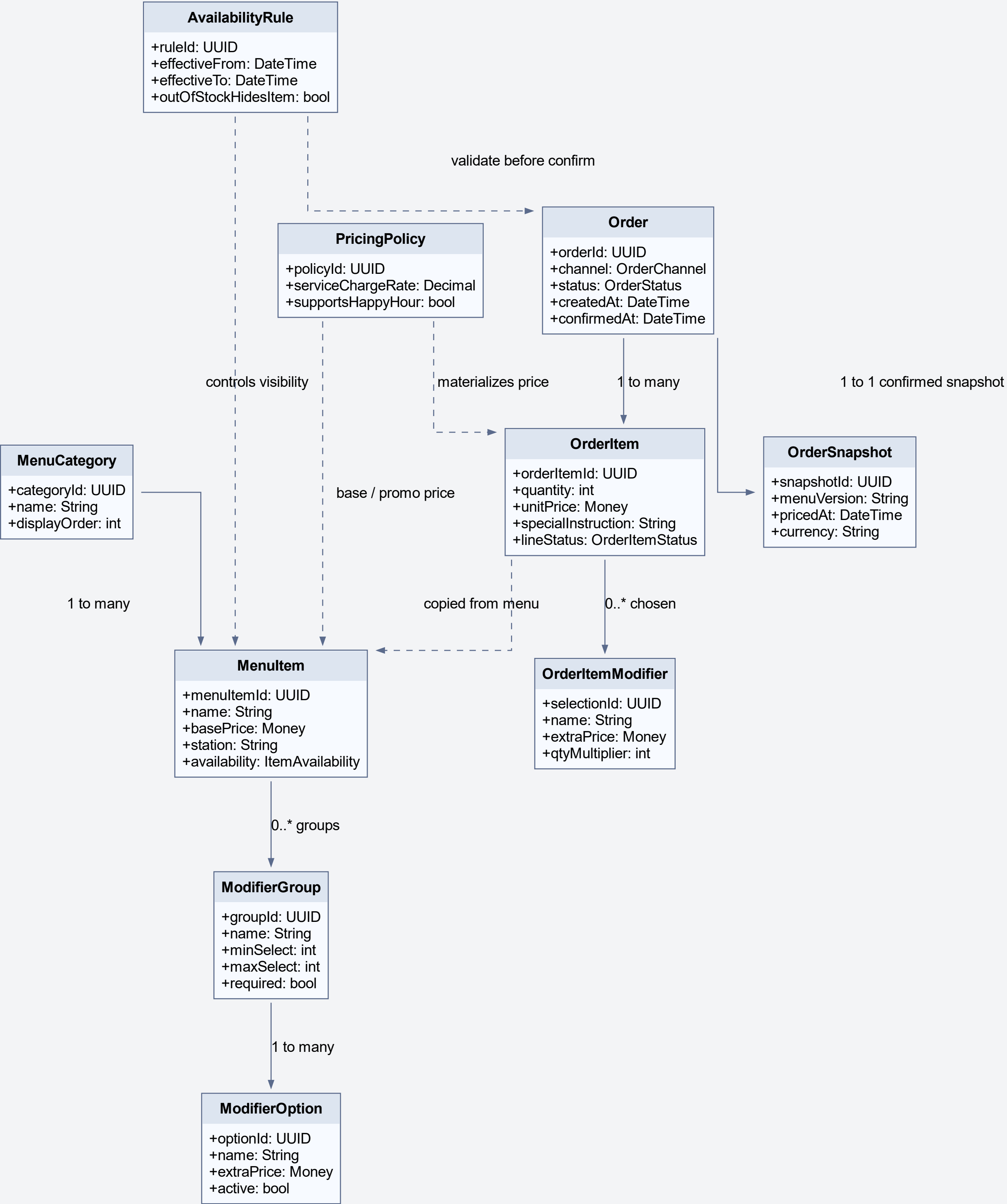
UML Class Diagram - Ordering & Menu Service
