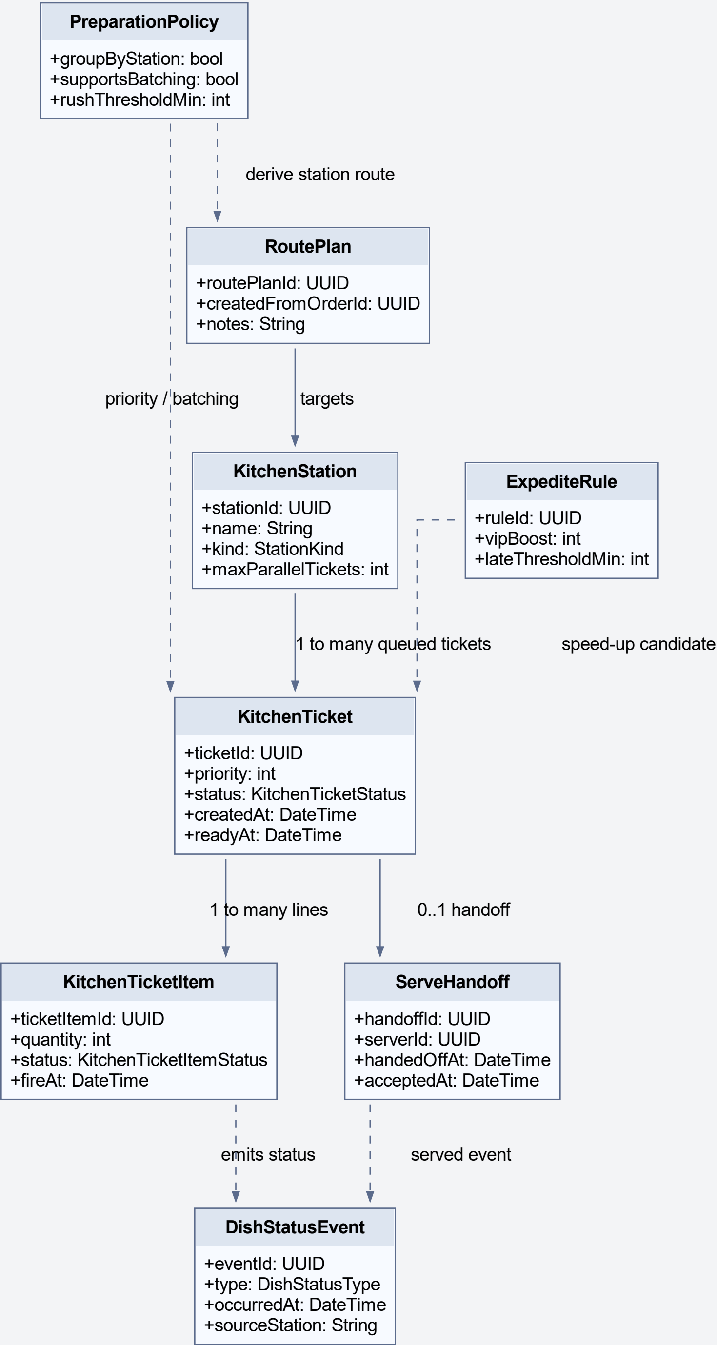
UML Class Diagram - Kitchen Coordination Service
