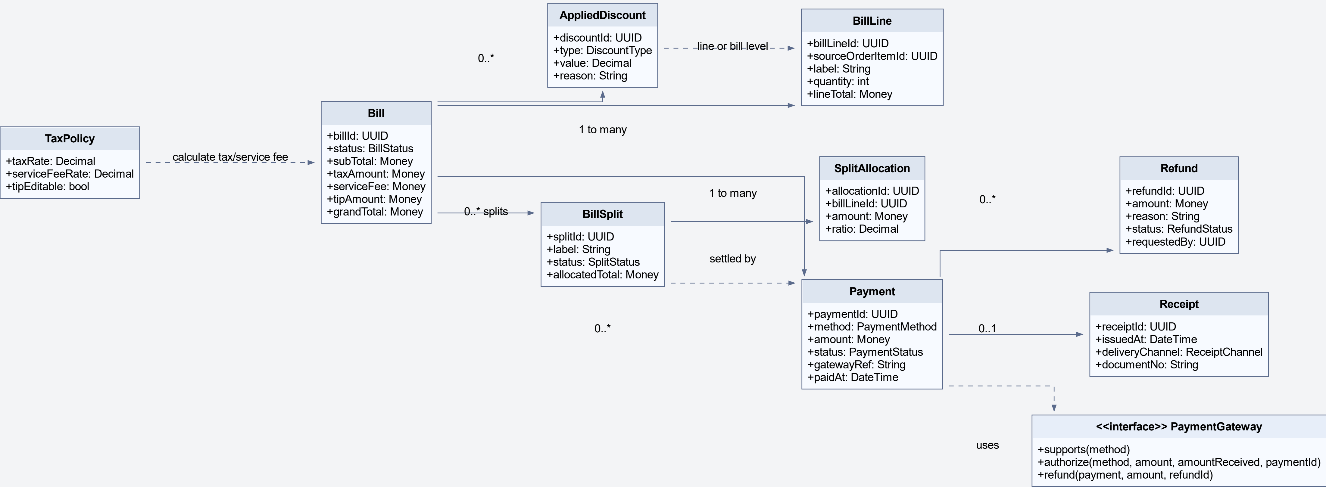
UML Class Diagram - Billing & Settlement Service
