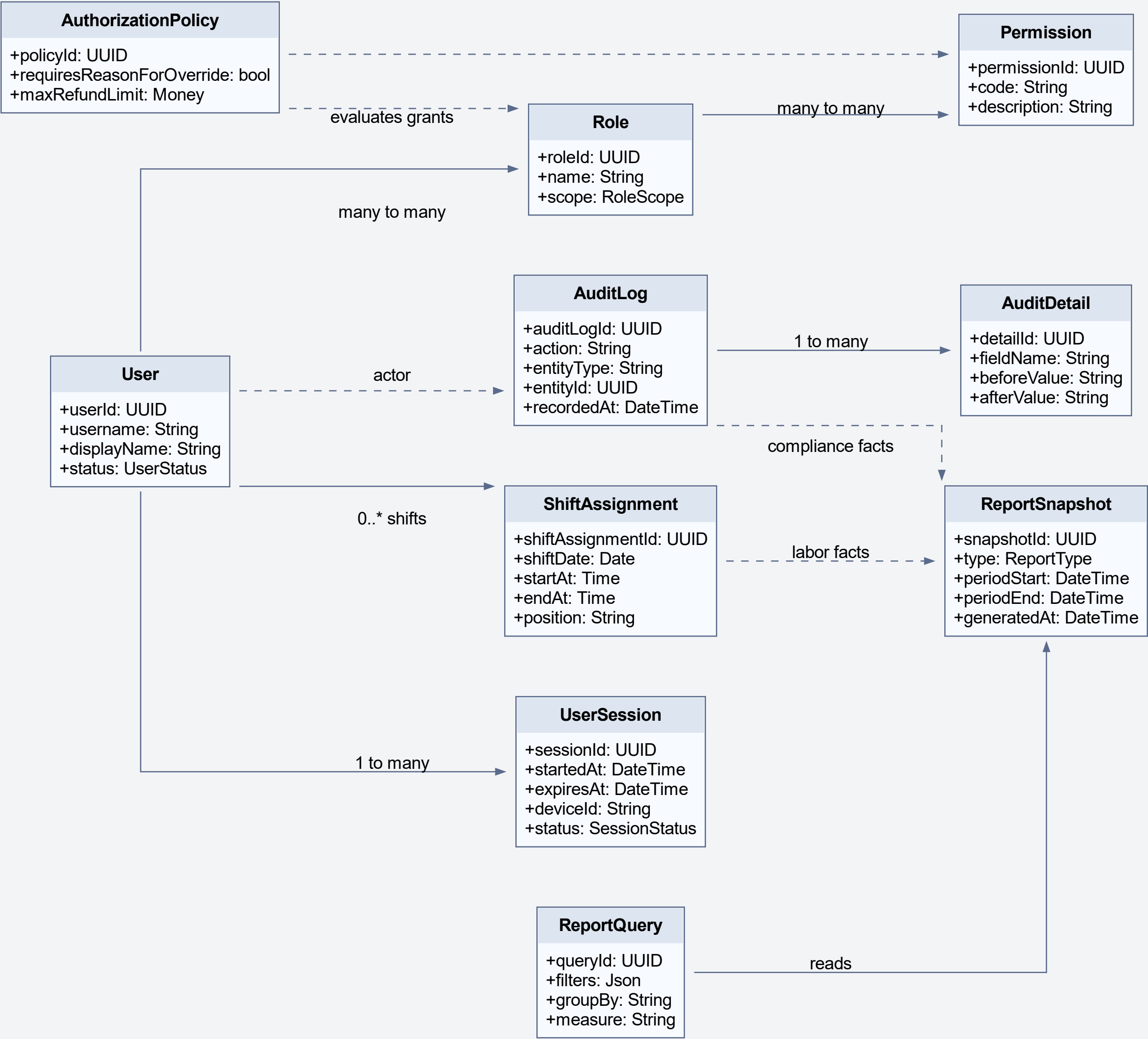
UML Class Diagram - IAM & Audit Service and Reporting Service
