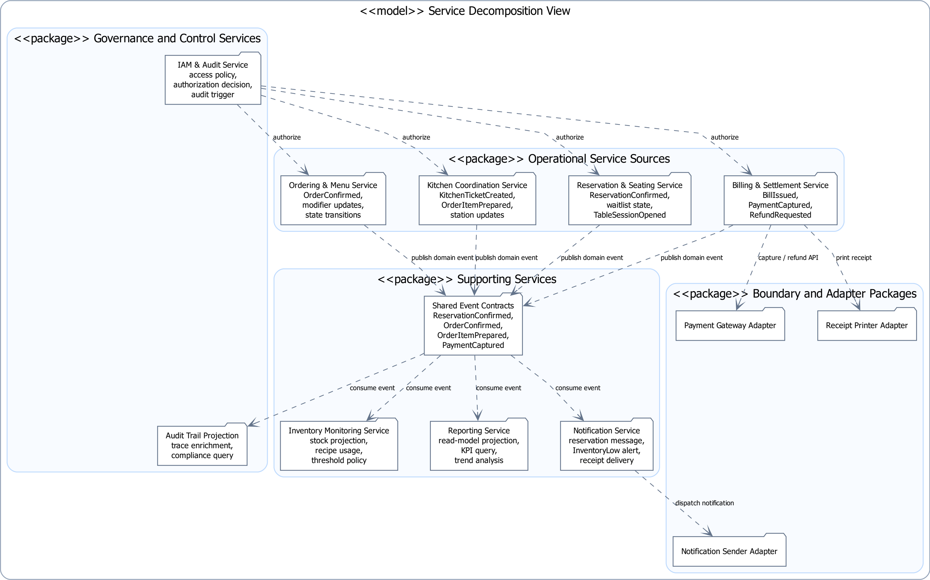
UML Package Diagram - Supporting and Cross-Cutting Services of IRMS
