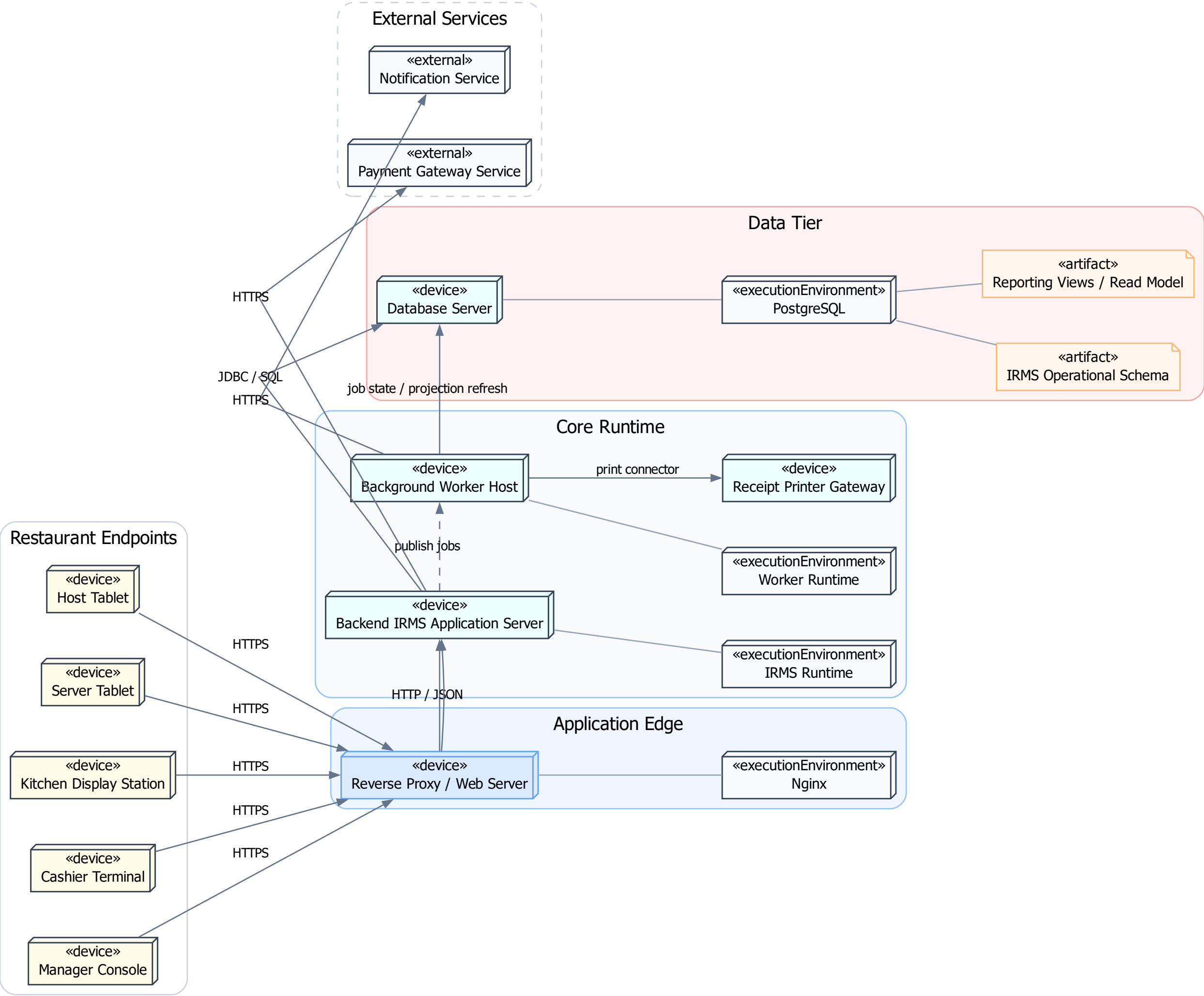
Deployment Diagram - Physical Deployment Overview
