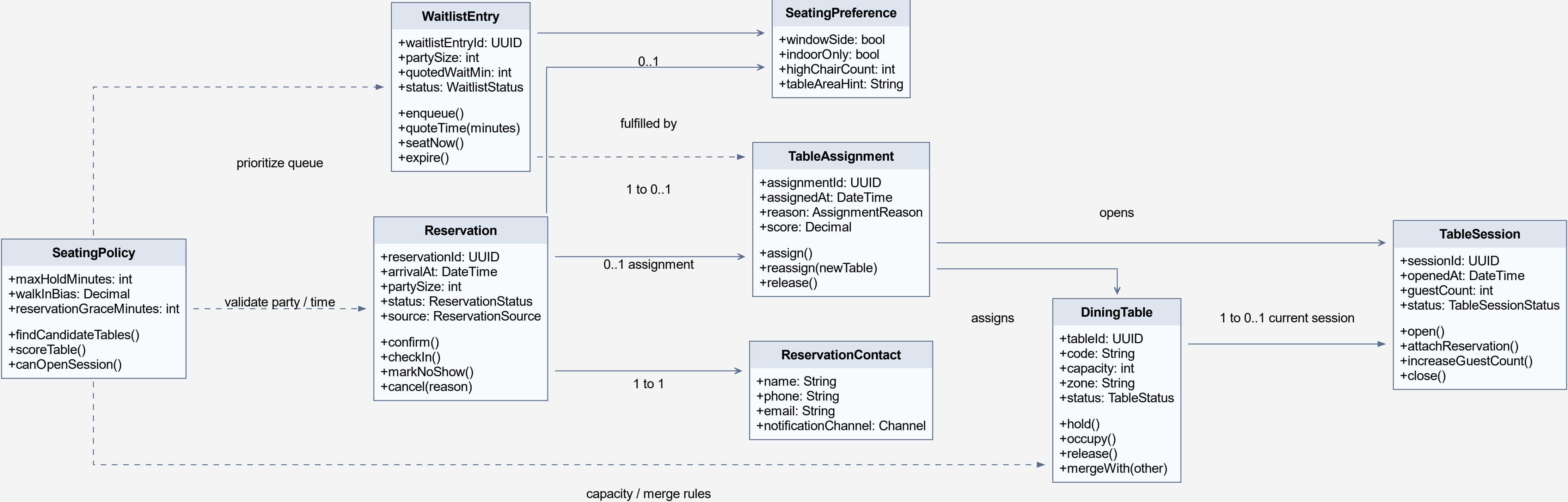
UML Class Diagram - Reservation & Seating Service
