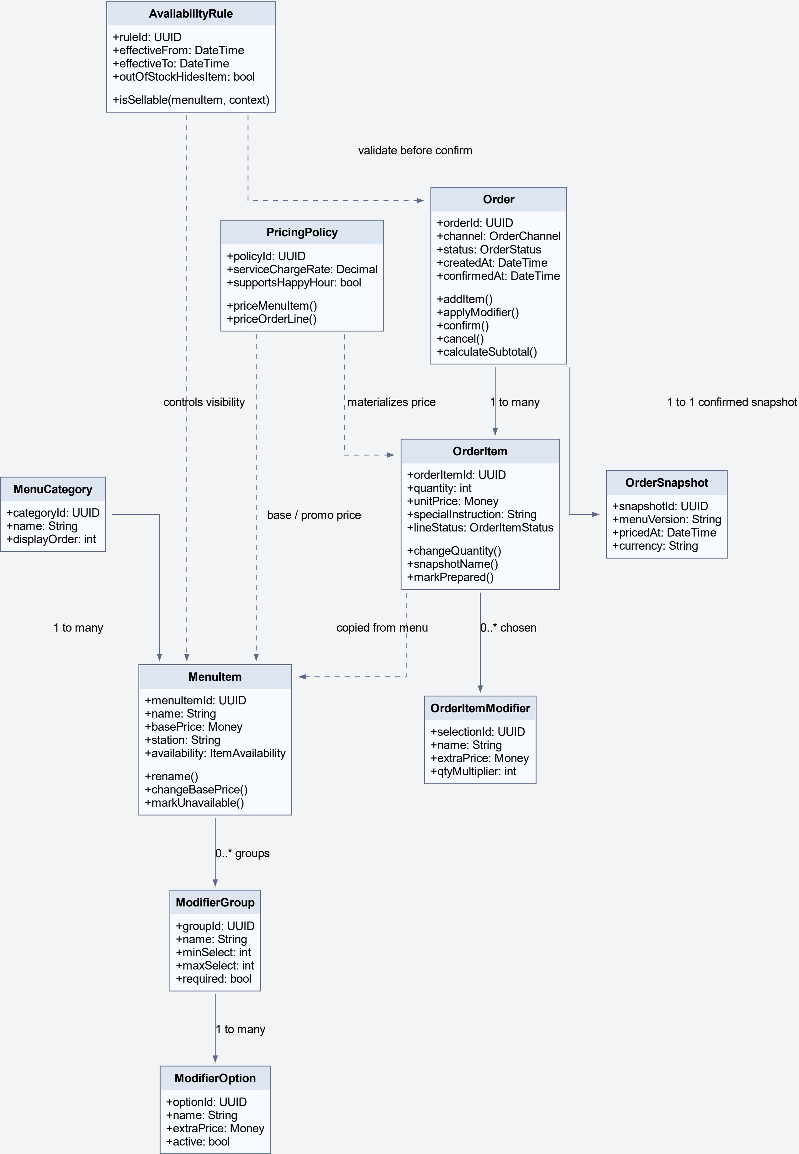
UML Class Diagram - Ordering & Menu Service
