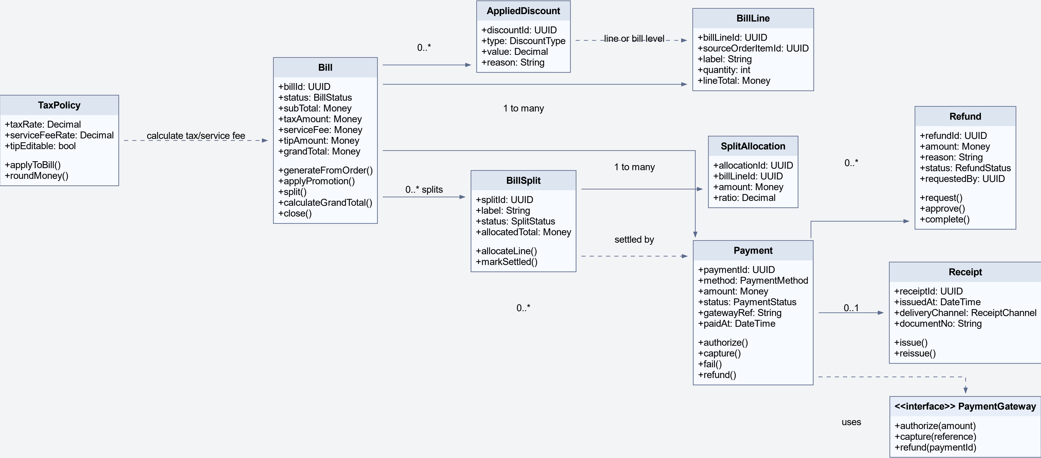
UML Class Diagram - Billing & Settlement Service
