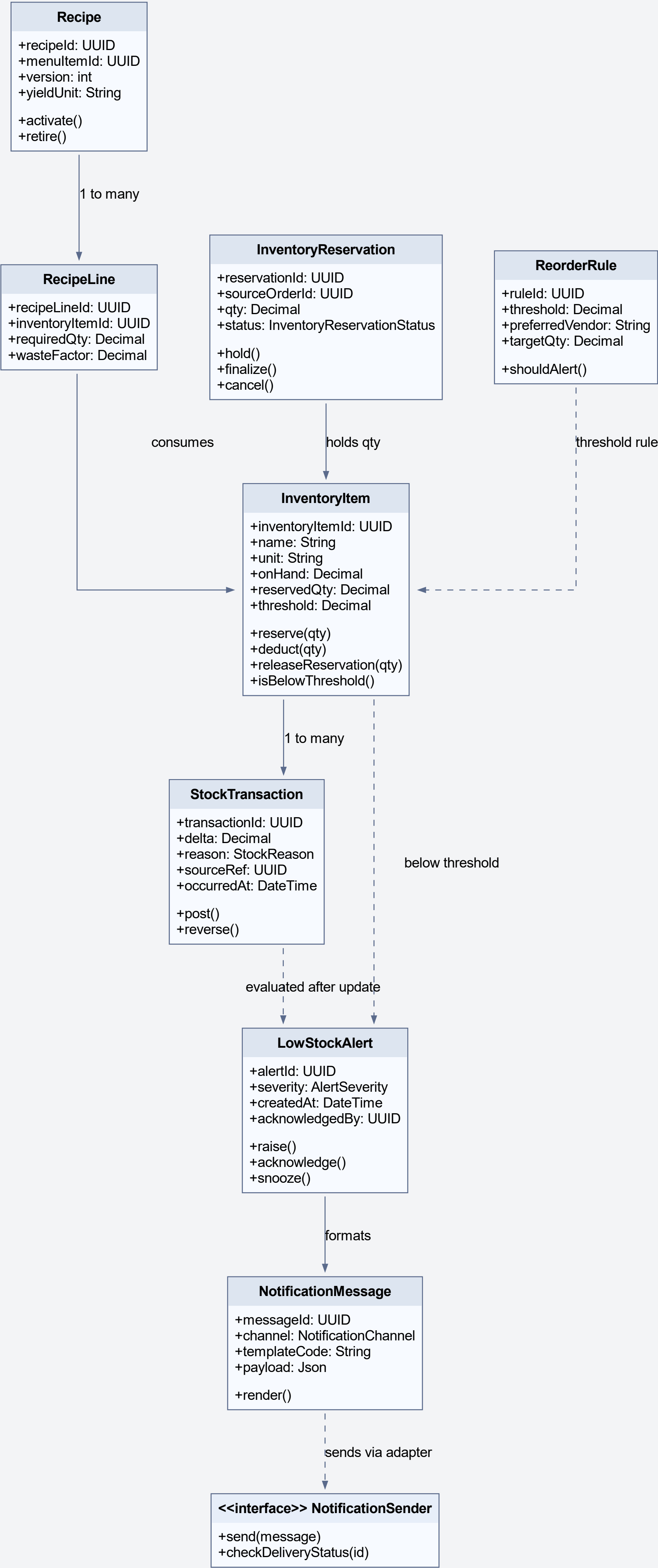
UML Class Diagram - Inventory Monitoring Service and Notification Service
