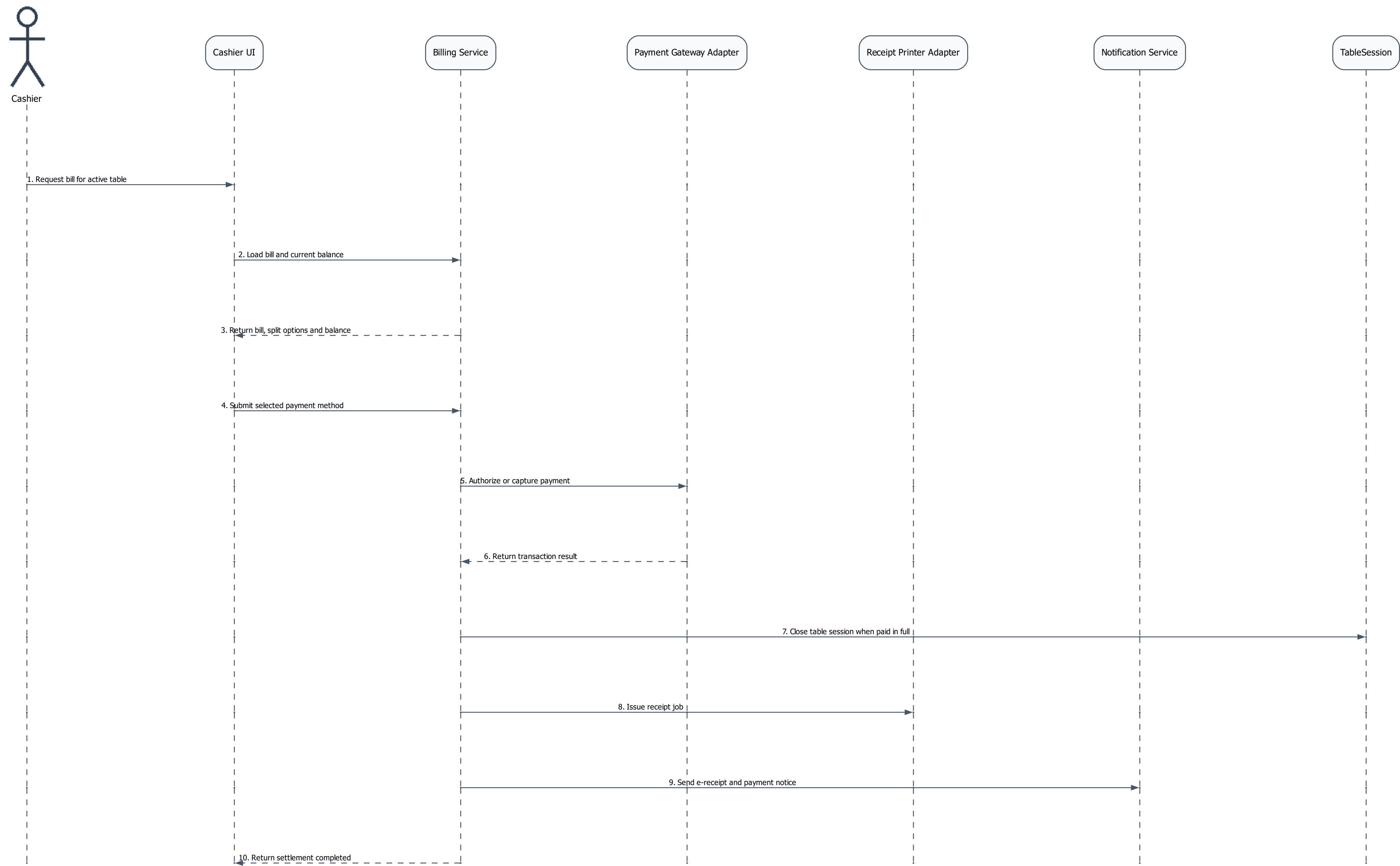
UML Sequence Diagram - Checkout, Payment and Receipt
