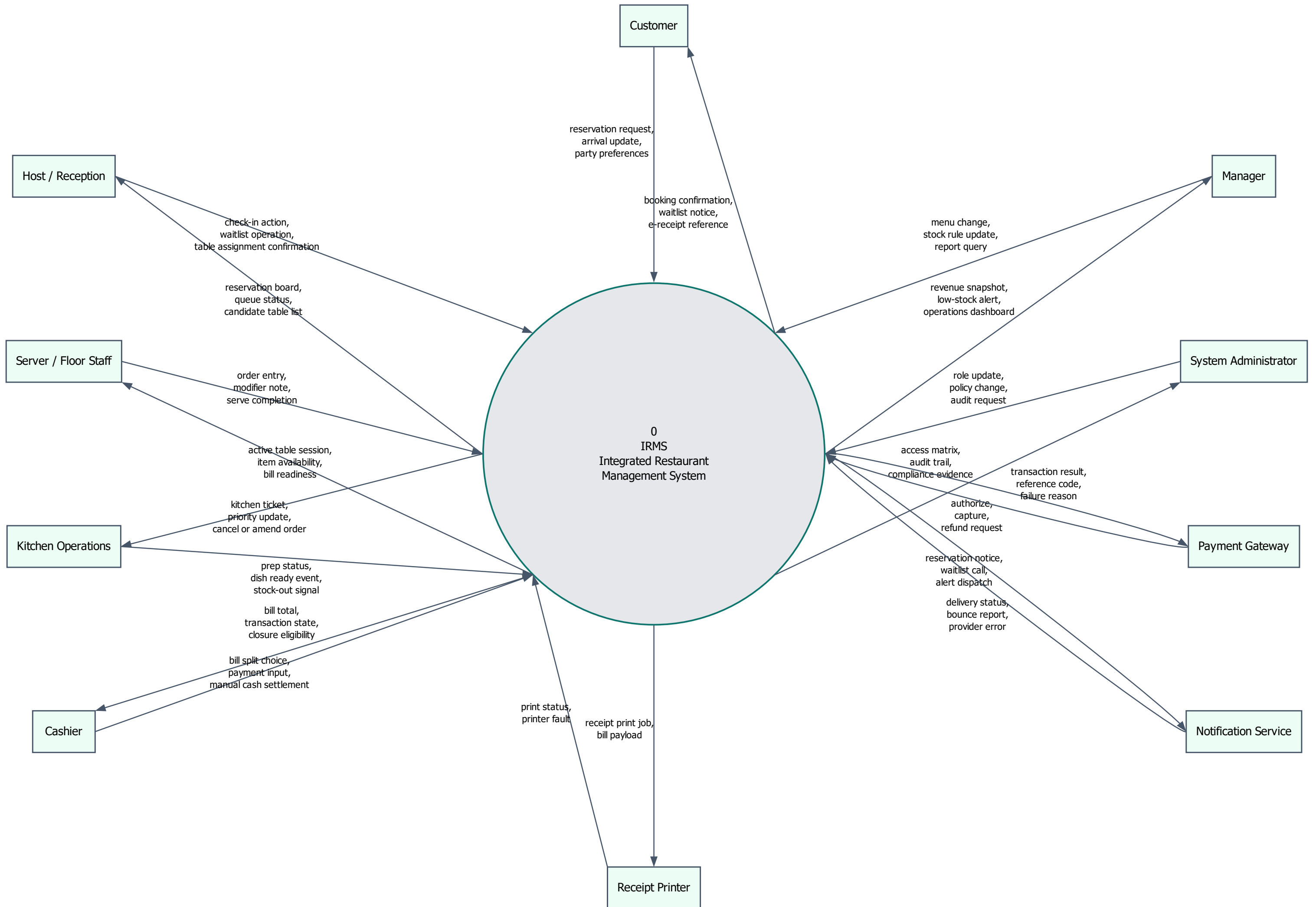
System Context Diagram - IRMS
