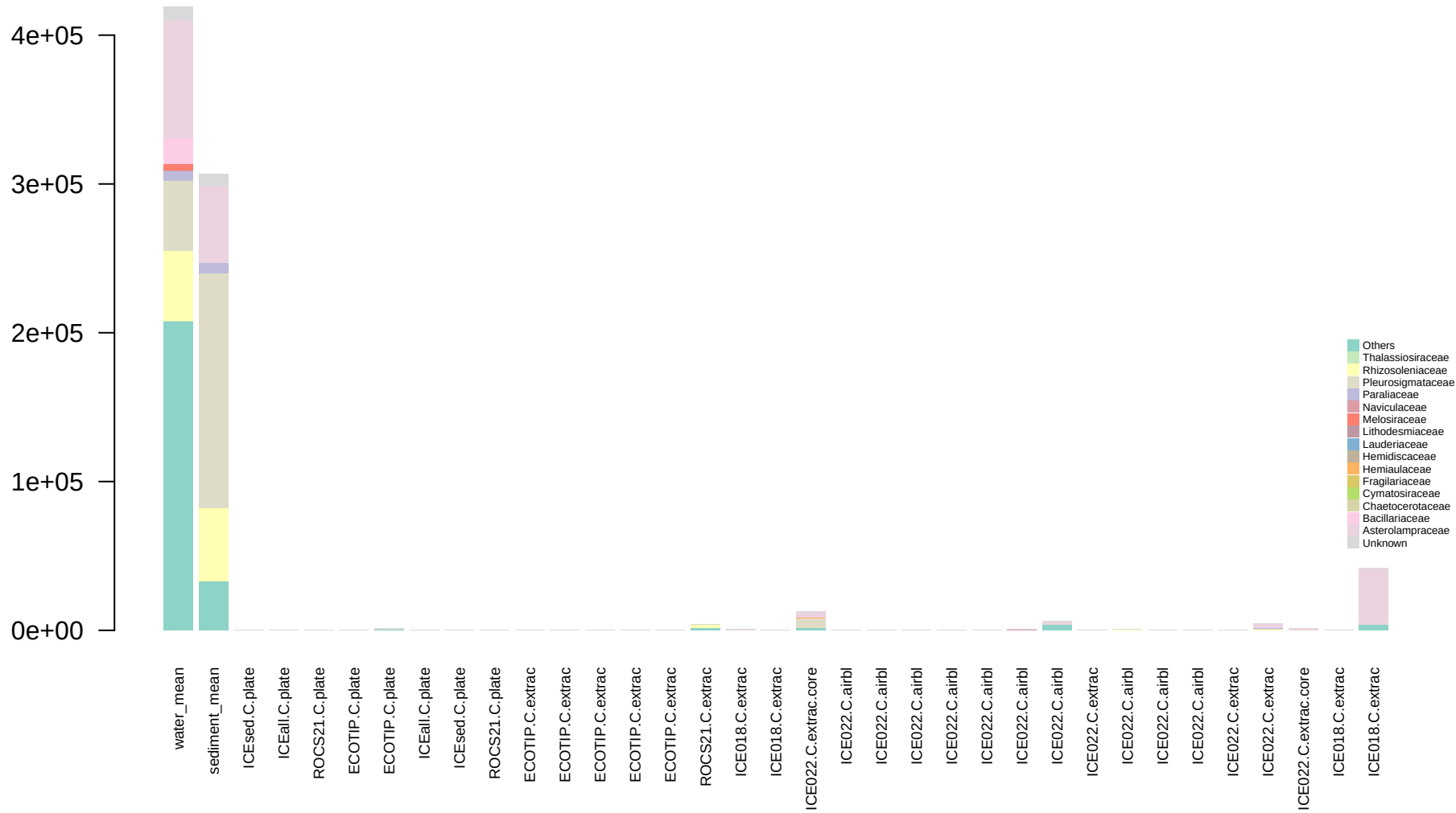
Read Abundance
