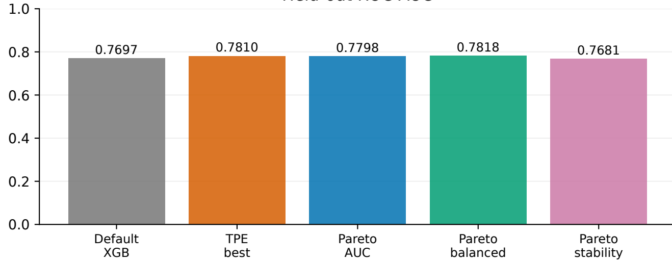
Held-out ROC-AUC
