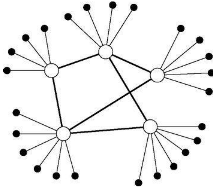
Figure 19.1: The structure of a peer-to-peer network with supernodes. Client nodes (filled circles) are connected to a network of supernodes (open circles) that have aboveaverage network bandwidth and hence can conduct searches quickly.
