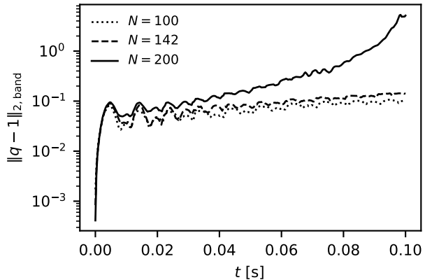
(a) baseline: band gradient error
