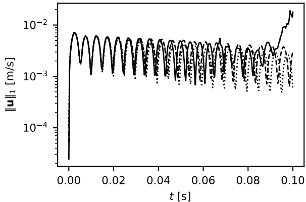
(b) baseline: velocity (the oscillation)
