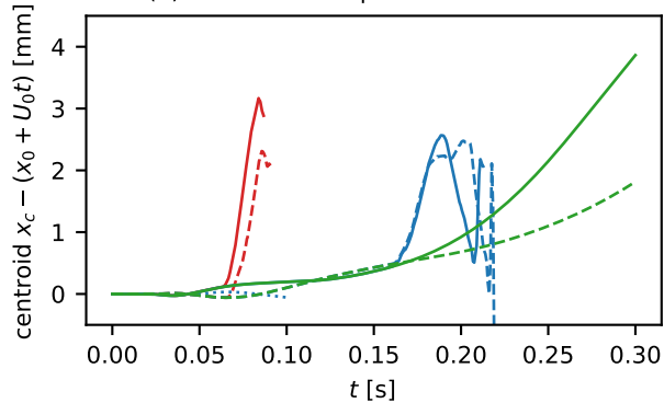
(b) lead of the droplet over the stream
