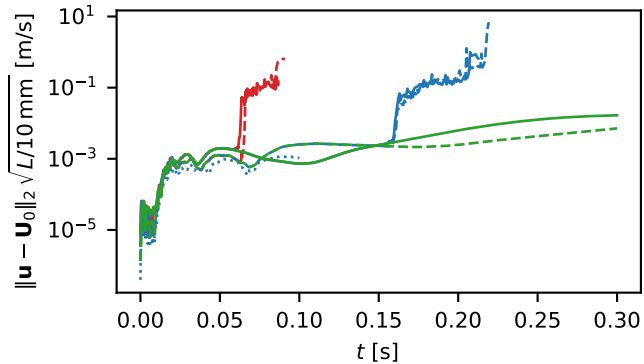
(a) spurious current, three box lengths
