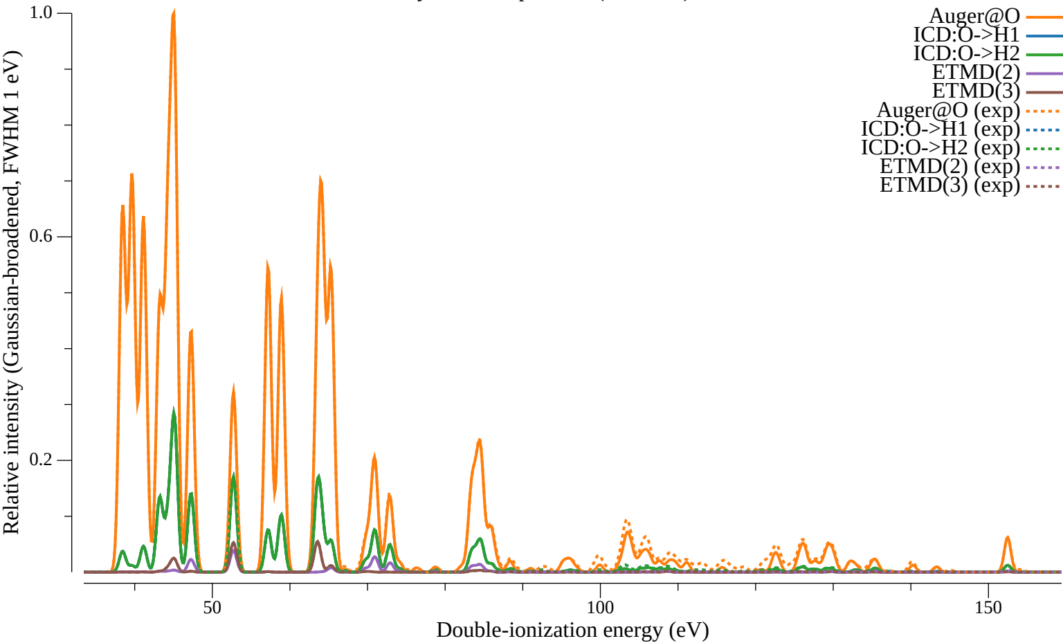
Decay-channel spectrum (initial: O)
